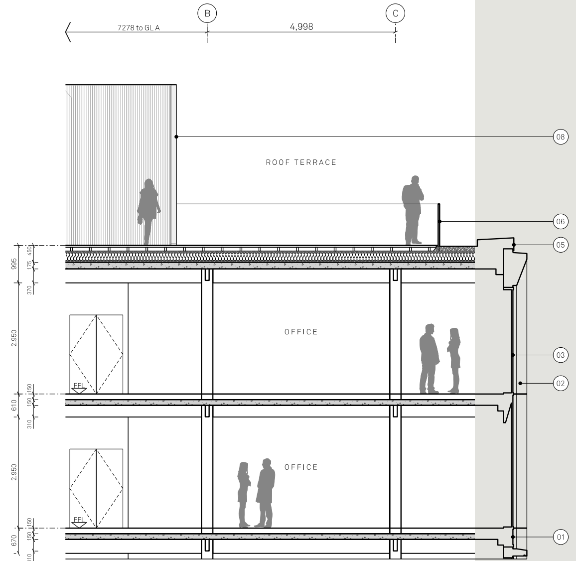
SECTION A Office Levels and Roof Terrace
