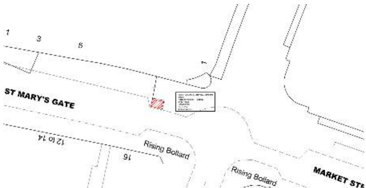
Fig 20: 2D drawing of the proposed location for a cycle hire station
