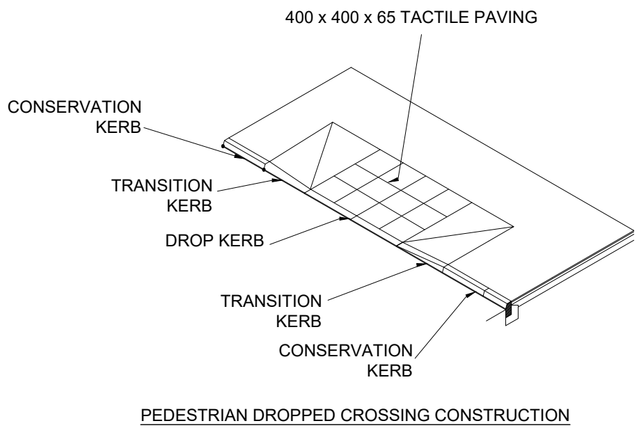
PEDESTRIAN DROPPED CROSSING CONSTRUCTION
