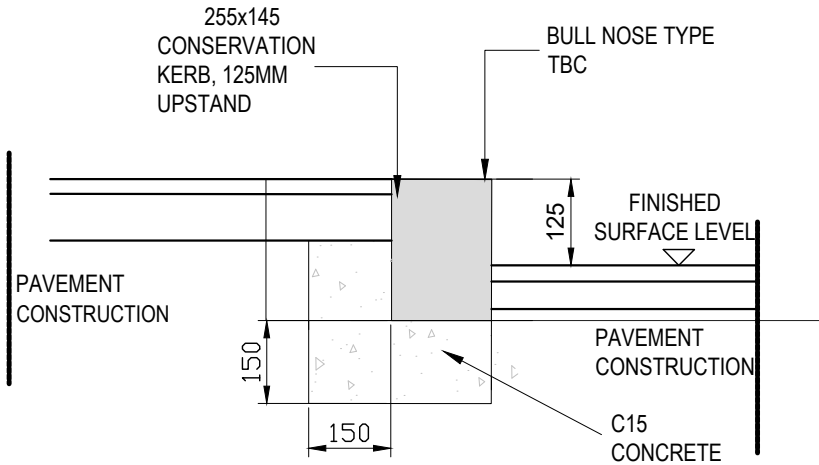
CK - CONSERVATION KERB DETAIL KERB BASE, BACKING AND KERB LAID AT SAME TIME
