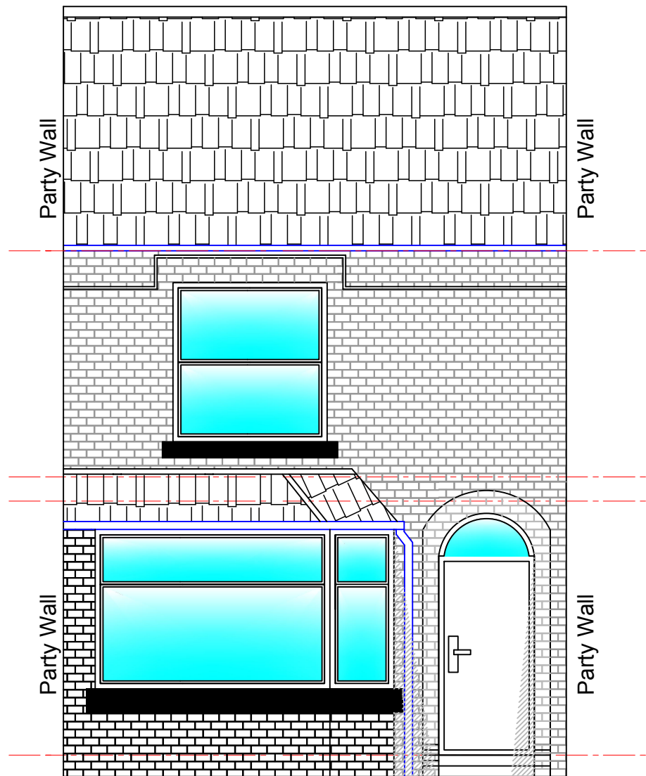
EXISTING FRONT ELEVATION 1:50 @ A1
