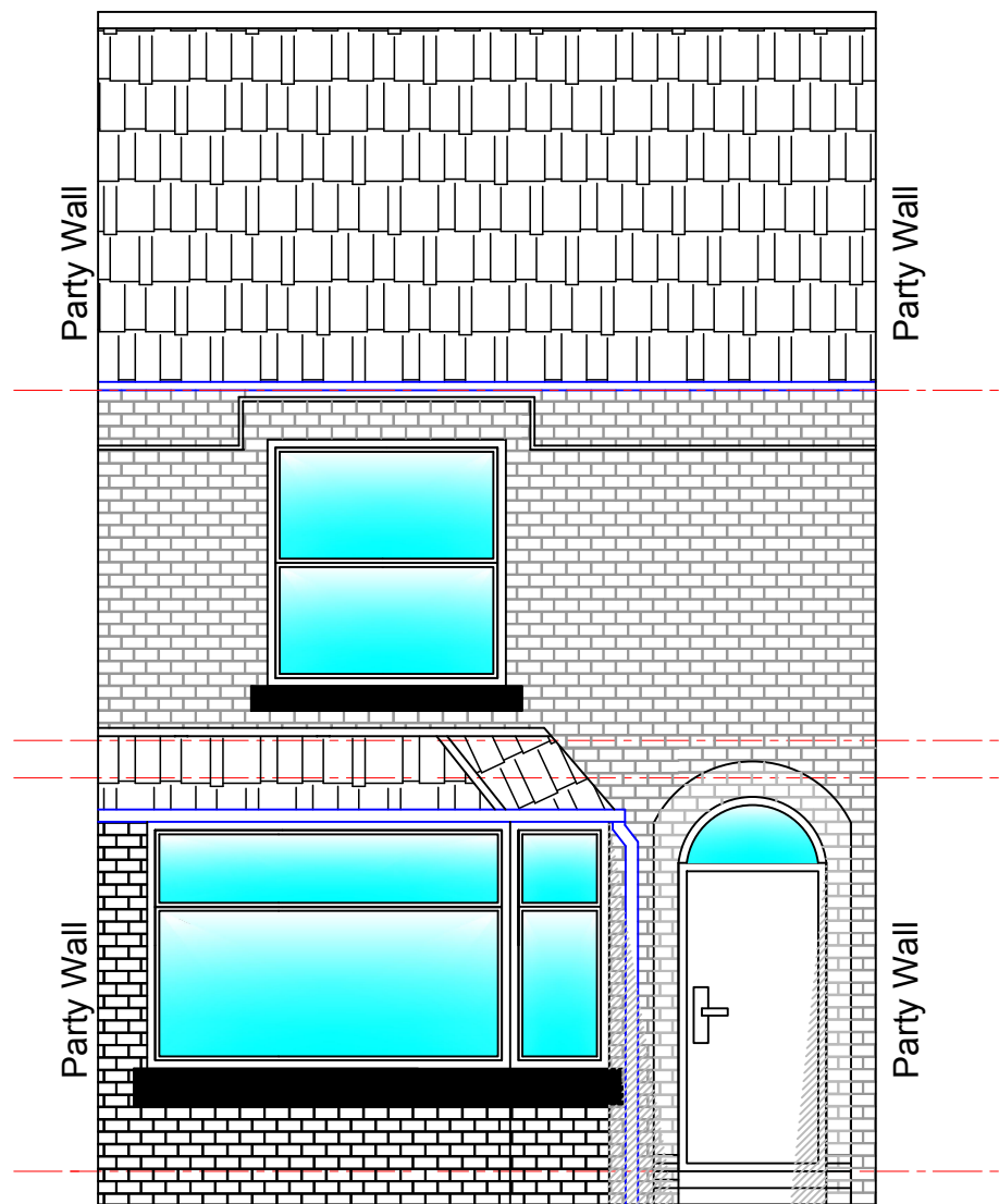
PROPOSED FRONT ELEVATION 1:50 @ A1
