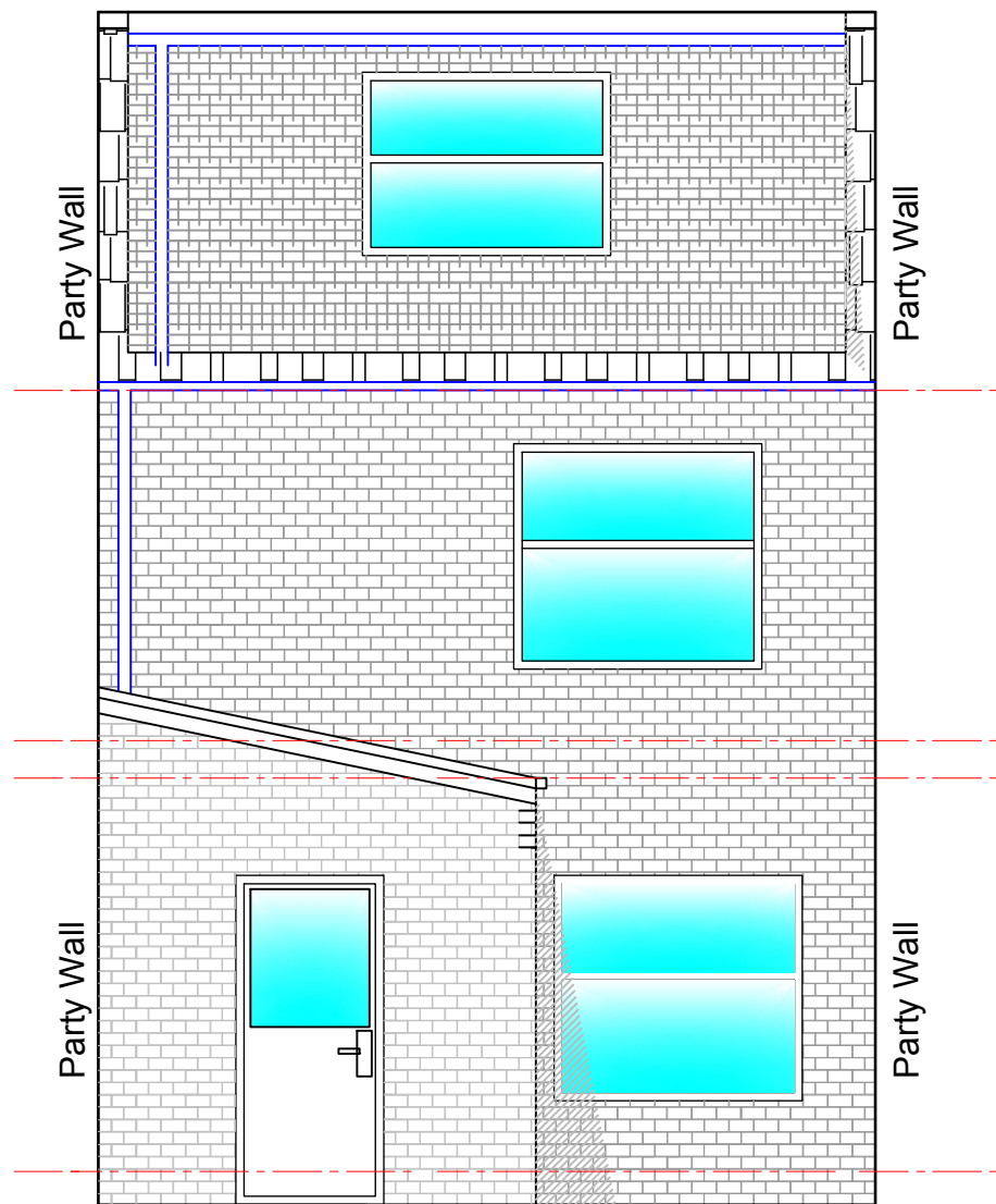
PROPOSED REAR ELEVATION 1:50 @ A1
