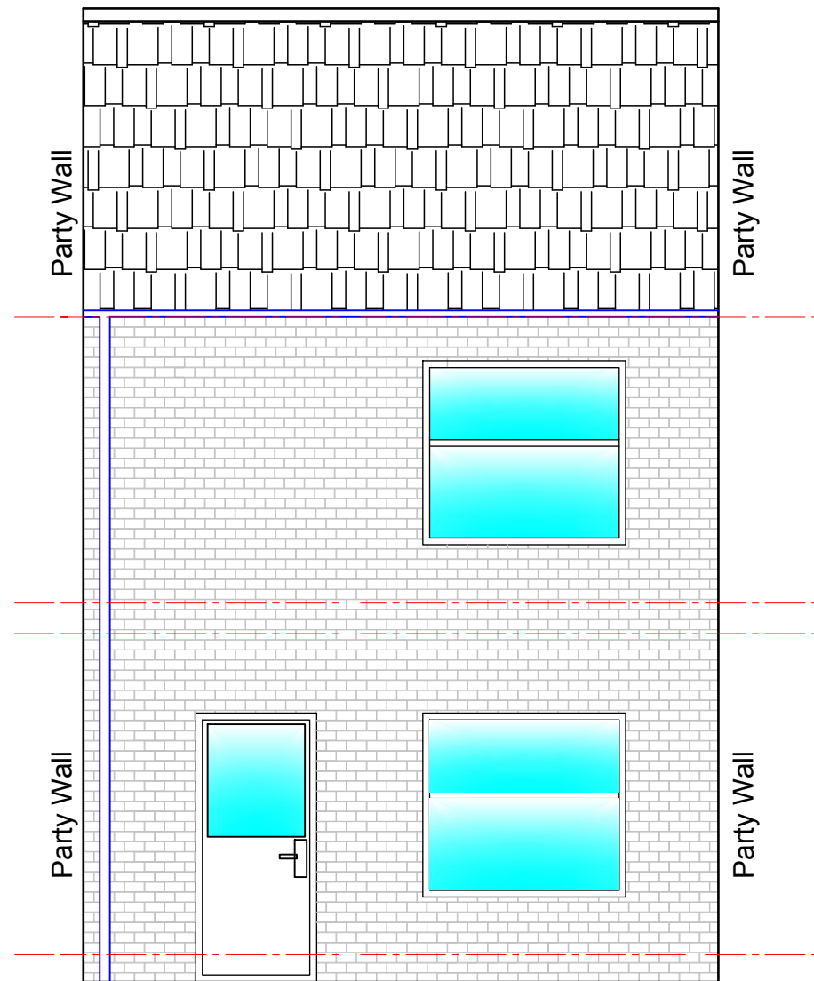
EXISTING REAR ELEVATION 1:50 @ A1
