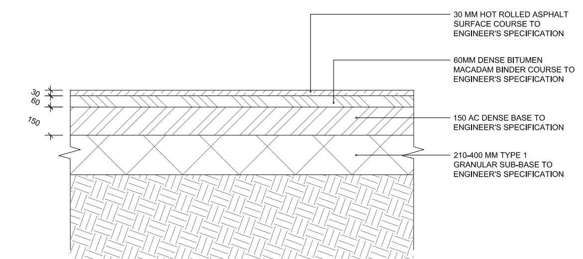
08 301 SECTION HOT ROLLED ASPHALT TO FOOTPATH
