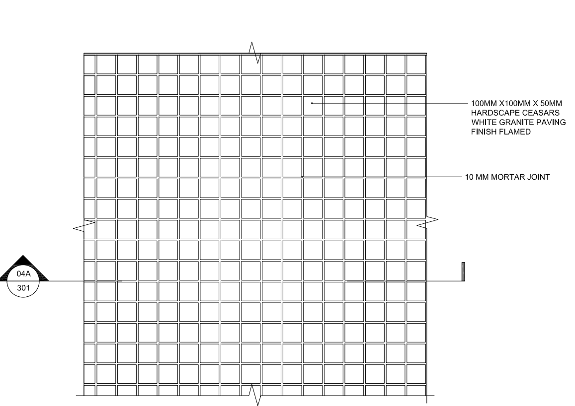
04B 301 PLAN HARDSCAPE ROYAL WHITE GRANITE PAVING
