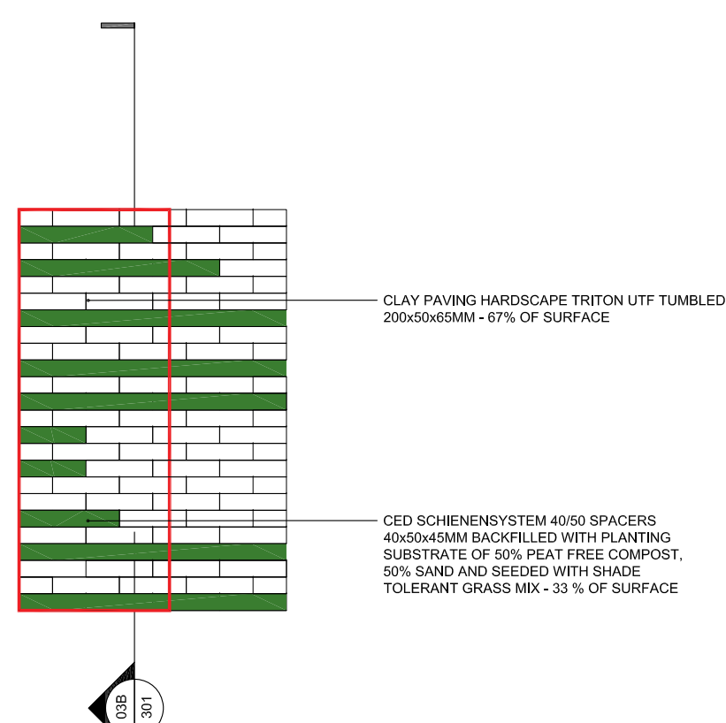
03B 301 SECTION GREEN PAVING - AREA 03
