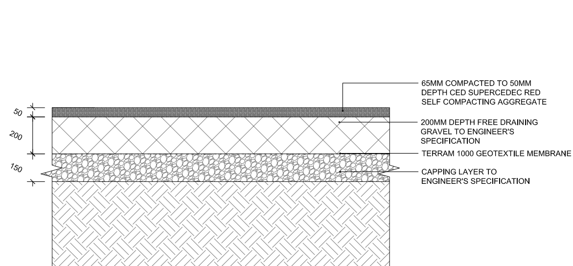
05 301 SECTION SUPERDEC SELF COMPACTING GRAVEL
