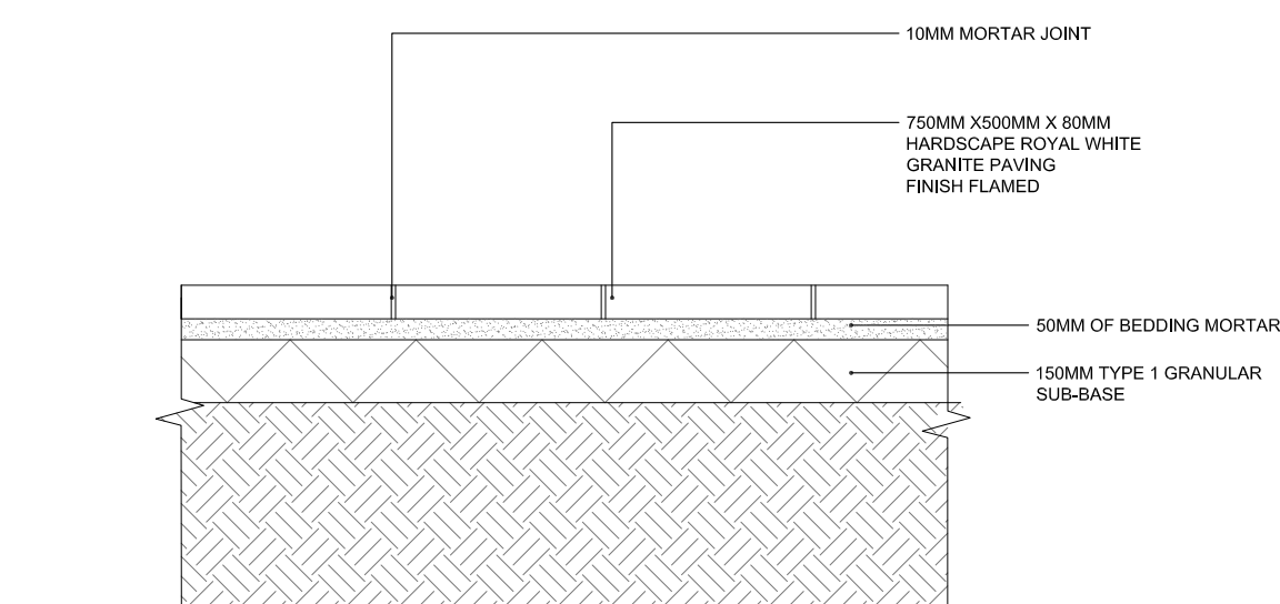
06A 301 PLAN HARDSCAPE ROYAL WHITE GRANITE PAVING
