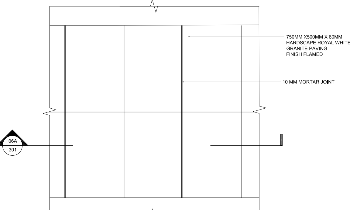
08B 301 PLAN HARDSCAPE ROYAL WHITE GRANITE PAVING
