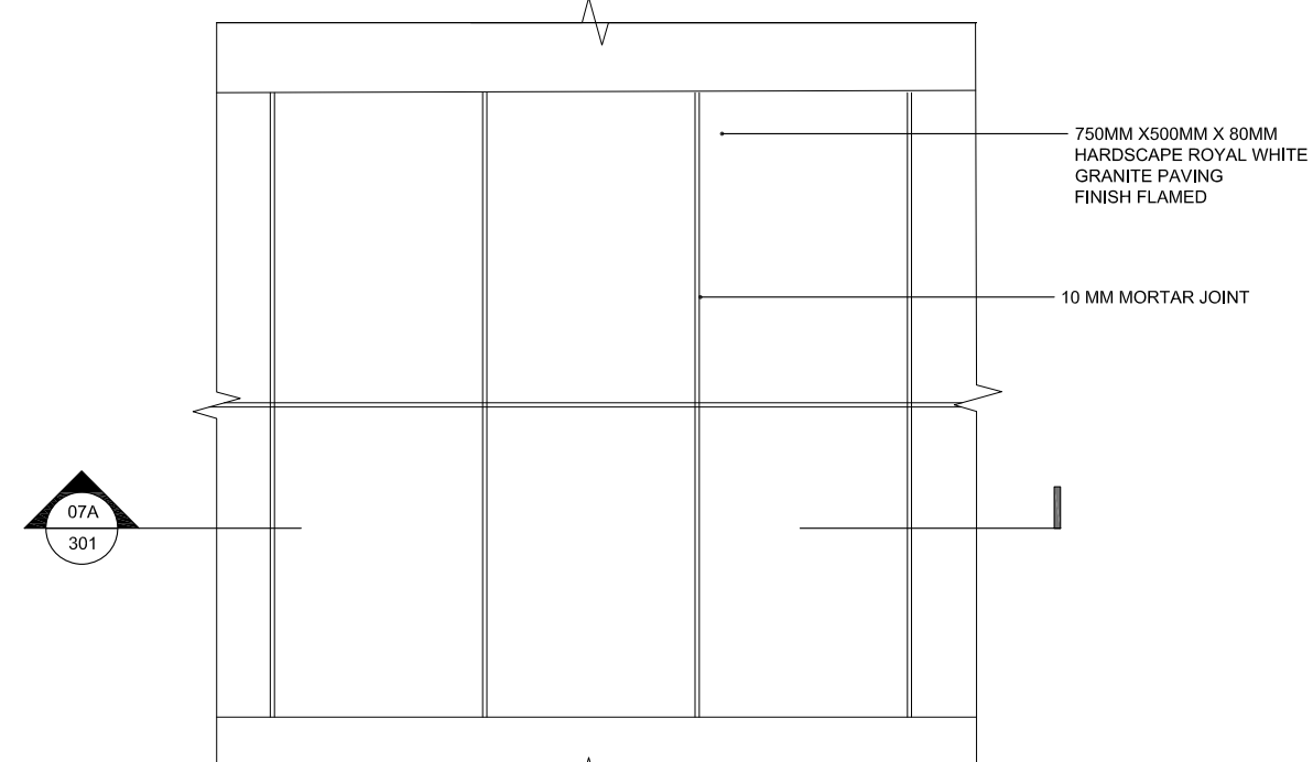
07B 301 PLAN HARDSCAPE ROYAL WHITE GRANITE PAVING
