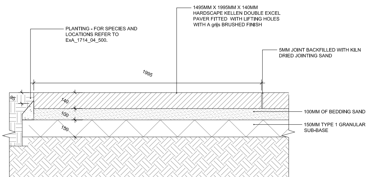
08A 301 SECTION HARDSCAPE KELLEN DOUBLE EXCEL SLAB PAVING
