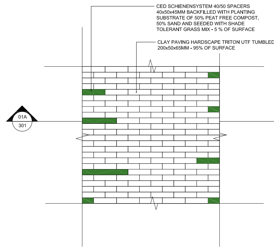
01B 301 PLAN GREEN PAVING - AREA 01
