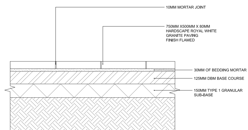
07A 301 SECTION HARDSCAPE ROYAL WHITE GRANITE PAVING (TRAFFICKED)
