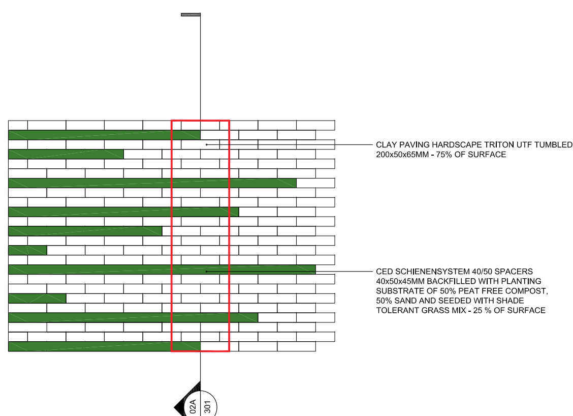
02B 301 PLAN GREEN PAVING - AREA 02
