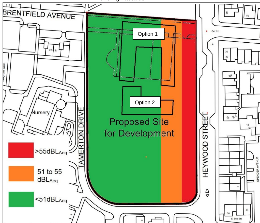
FIGURE 5.1 – Indicative Day-time Free-Field Ambient Noise Levels (dBL Aeq,30min ) Affecting Potential Building Facades
