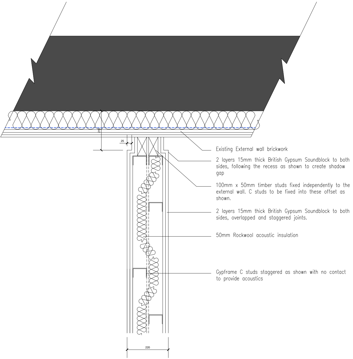
ACOUSTIC SHADOW GAP DETAIL
