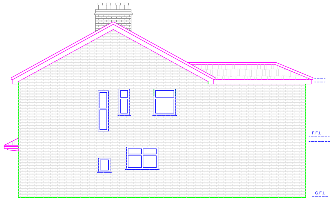
PROPOSED SIDE ELEVATION (NORTH)
