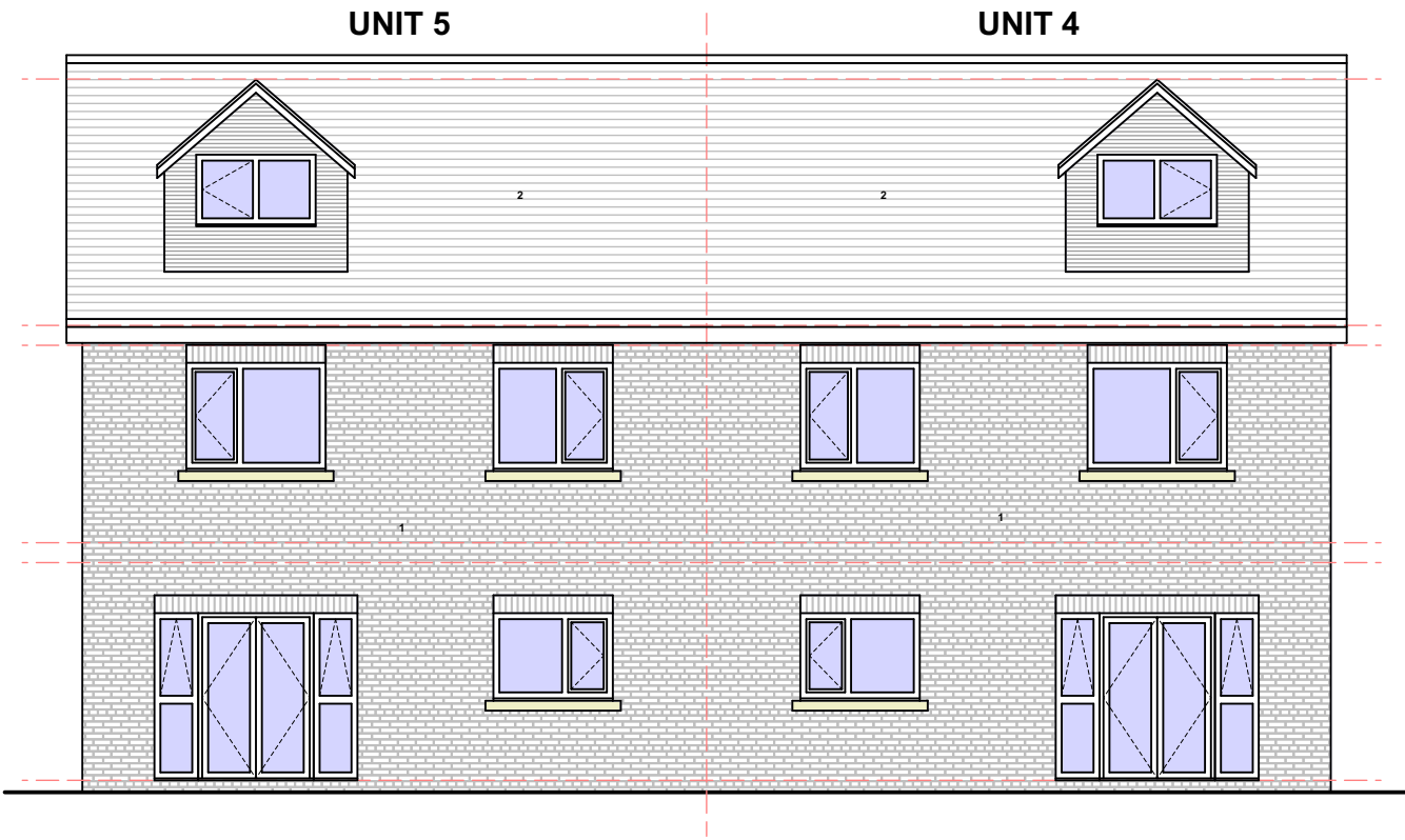
PROPOSED GA REAR ELEVATION UNITS 4-5
