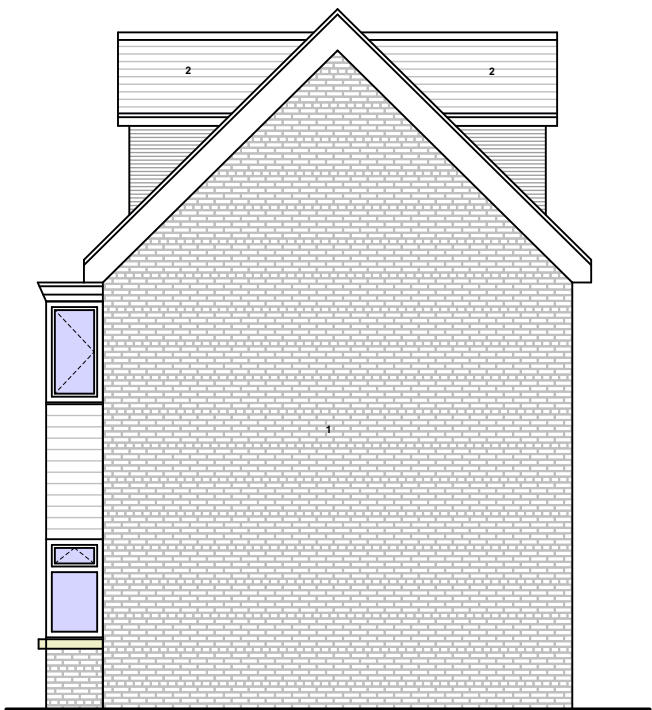
PROPOSED GA SIDE ELEVATION 1 UNITS 4-5
