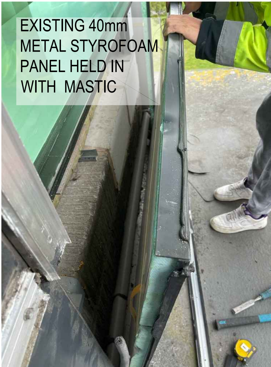
VIEW BEHIND PANEL
