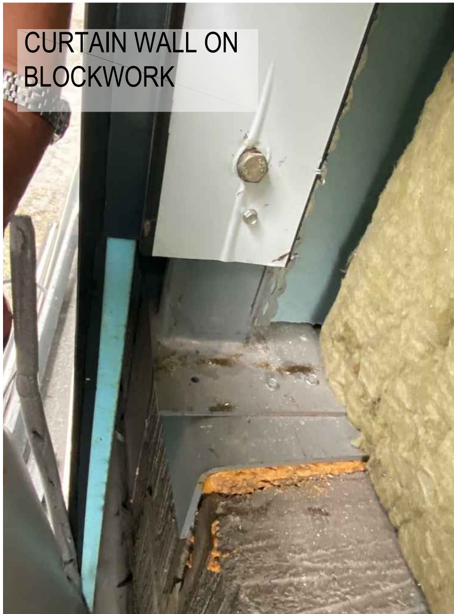
JUNCTION AT BASE DETAIL
