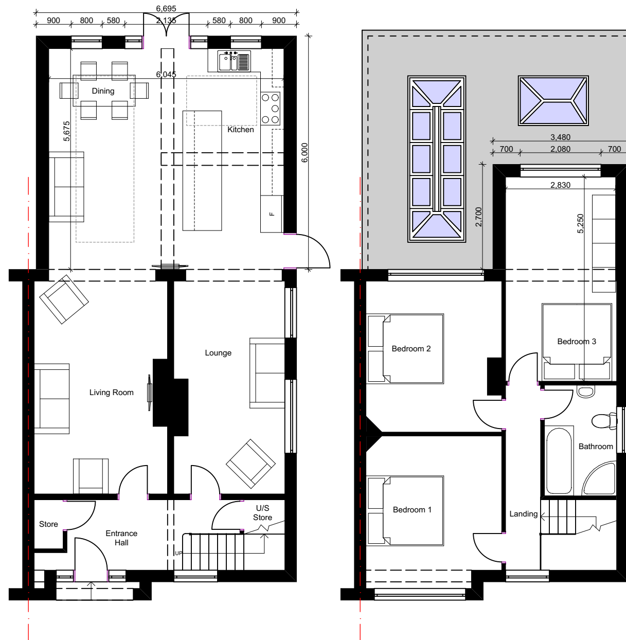
PROPOSED GA GROUND FLOOR
