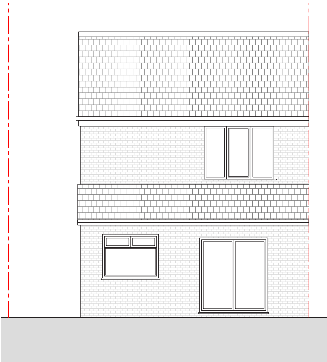
EXISTING REAR ELEVATION 1:100 @ A3
