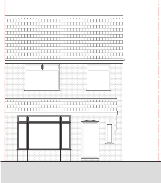
EXISTING FRONT ELEVATION 1:100 @ A3
