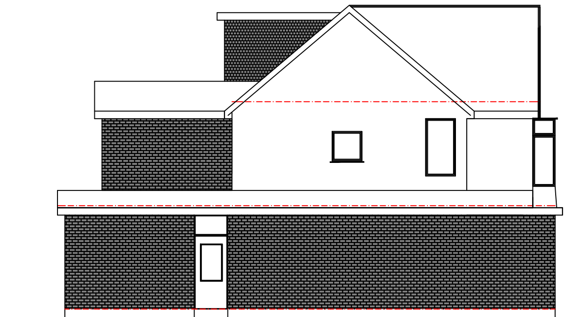
Side Elevation
