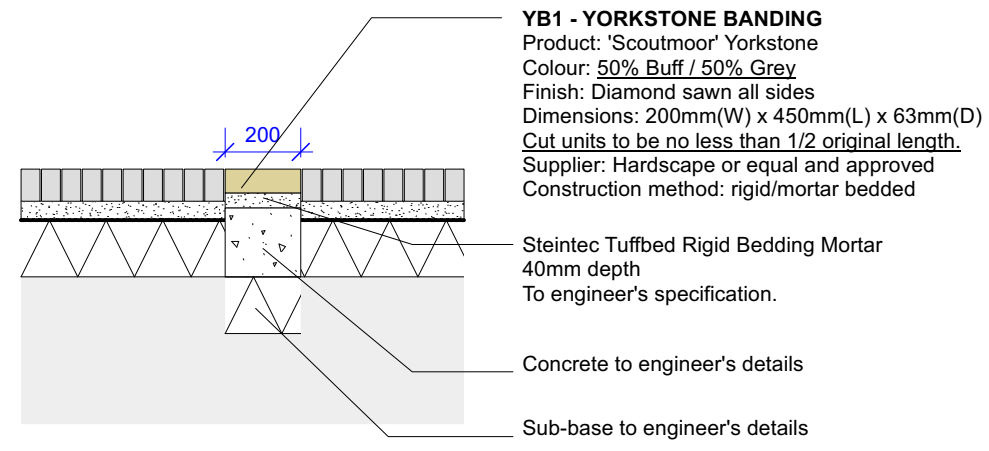
YB1 Yorkstone Banding - Off Podium Scale: 1:20
