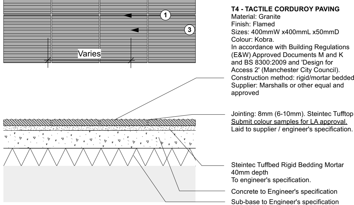
T4 Granite Tactile Corduroy Paving - to main square steps Scale: 1:20
