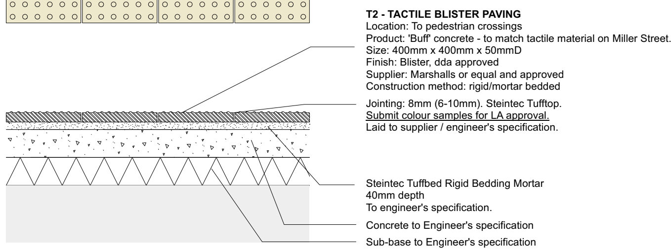
T2 Tactile Blister Paving - to crossings Scale: 1:20
