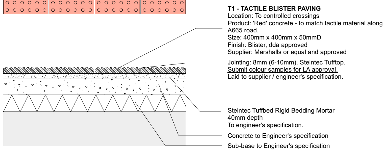
T1 Tactile Blister Paving - to controlled crossings Scale: 1:20
