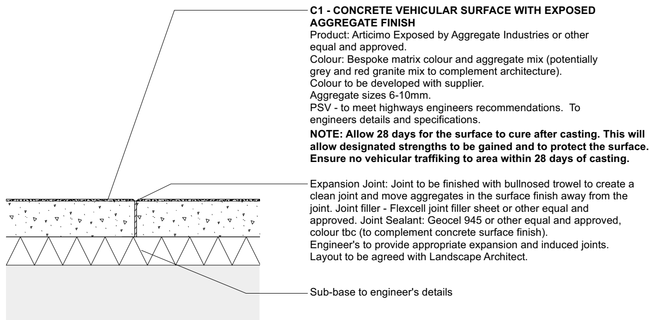
C1 In situ Concrete Surface - To Service Yard Scale: 1:20
