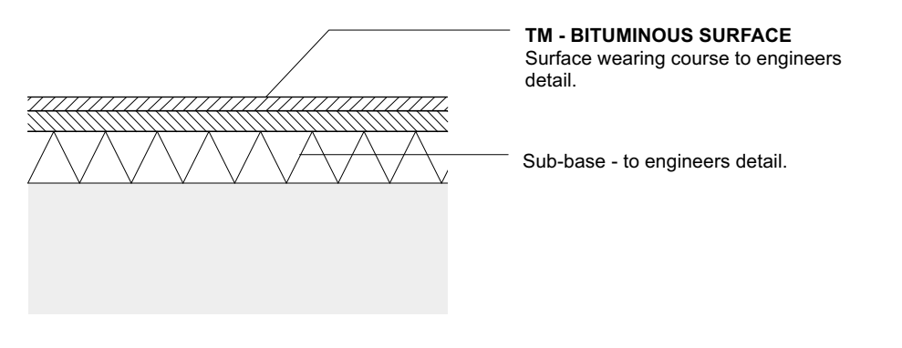
TM Bituminous surface - to highway Scale: 1:20
