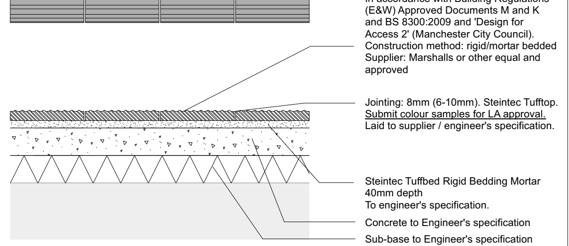
T3 PCC Tactile Corduroy Paving - to service yard steps Scale: 1:20
