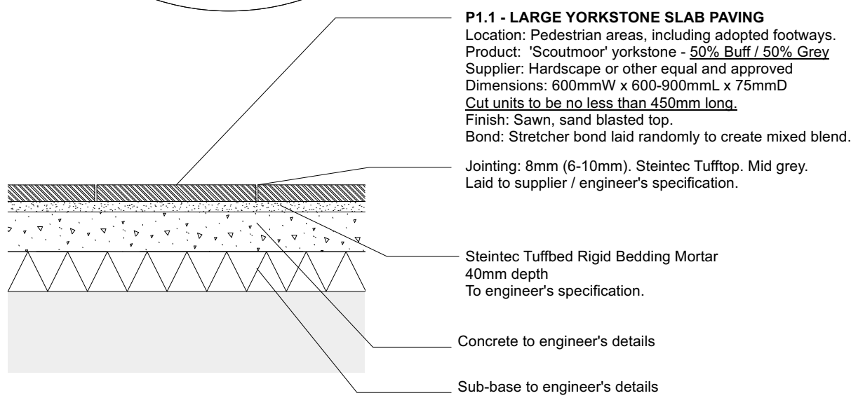
P1.1 Yorkstone Flags - to footpaths Scale: 1:20
