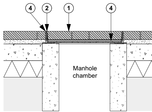
RM Recessed Manhole Cover Scale: 1:20
