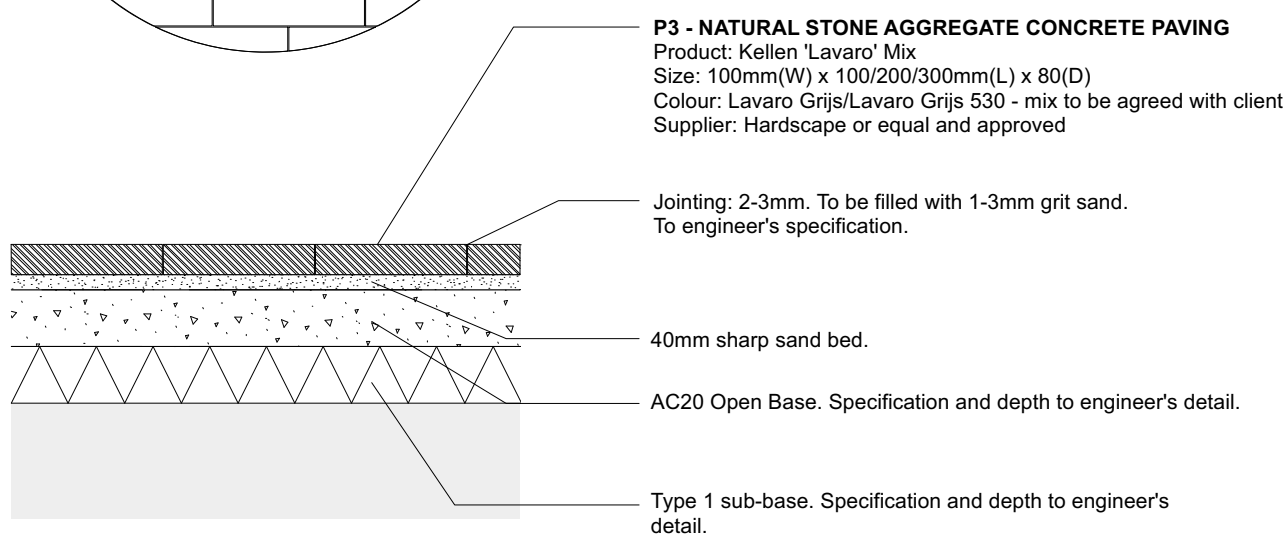
P3 Natural Stone Aggregate Concrete Block Paving Scale: 1:20
