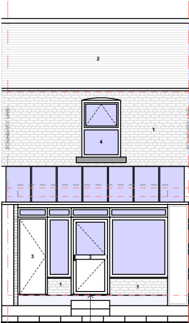
EXISTING GA FRONT ELEVATION @1:100
