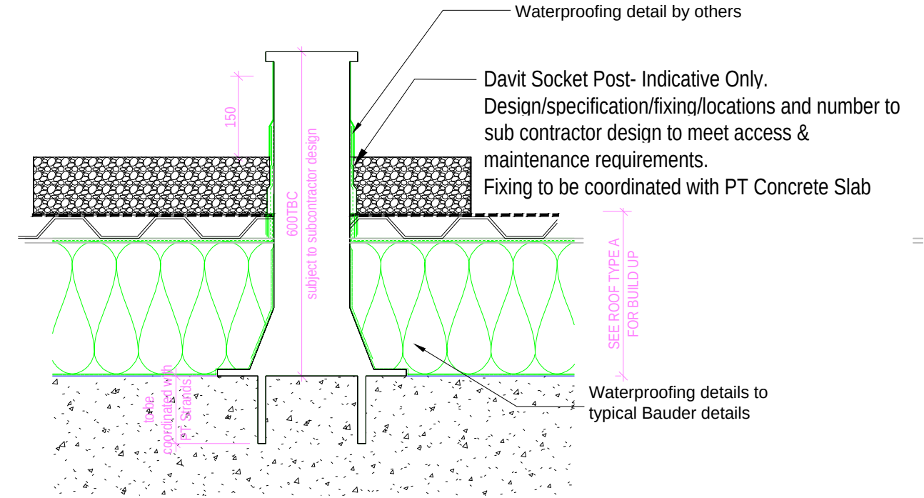
1:10 – Davit Detail
