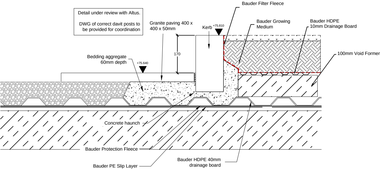
1:10 – Typical Lawn & Paving Detail
