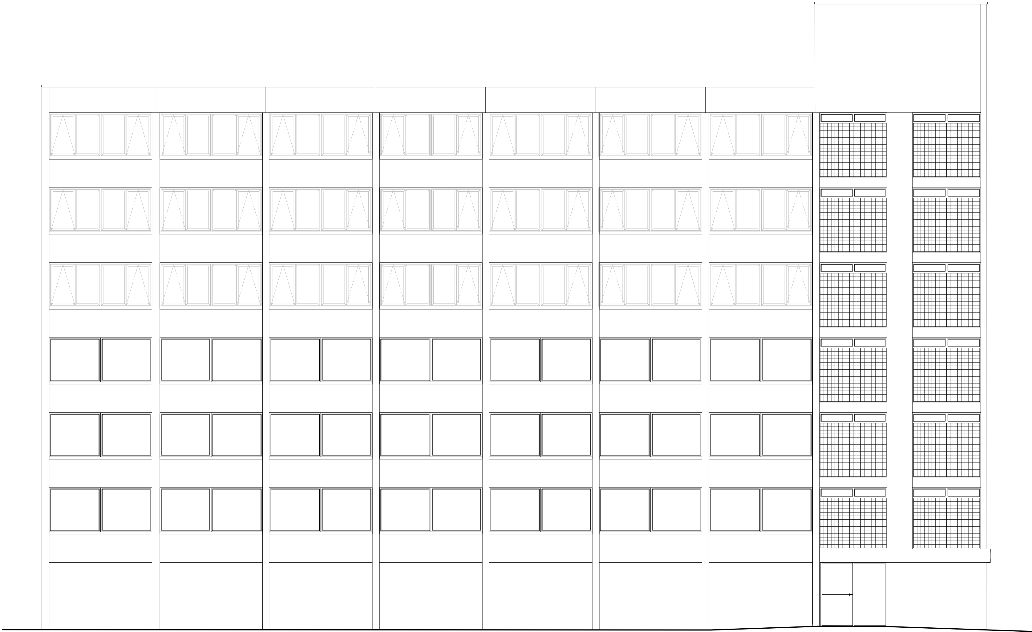
1 EXISTING ELEVATION A (SILVER ST) Scale: 1:100
