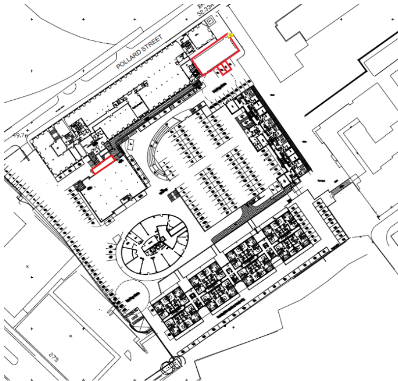
Figure 1: Site Plan
