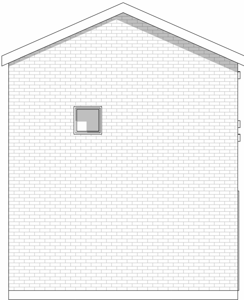
EXISTING REAR ELEVATION @1:50
