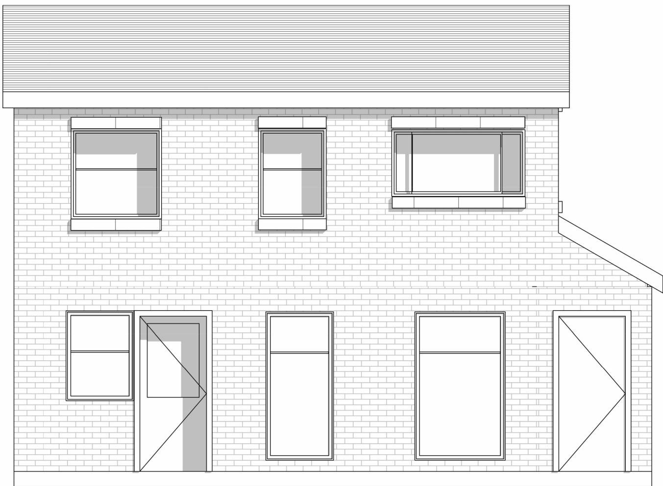
EXISTING LEFT ELEVATION @1:50
