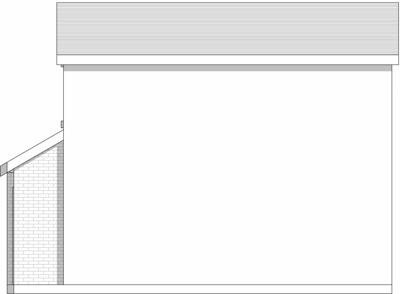
EXISTING RIGHT ELEVATION @1:50
