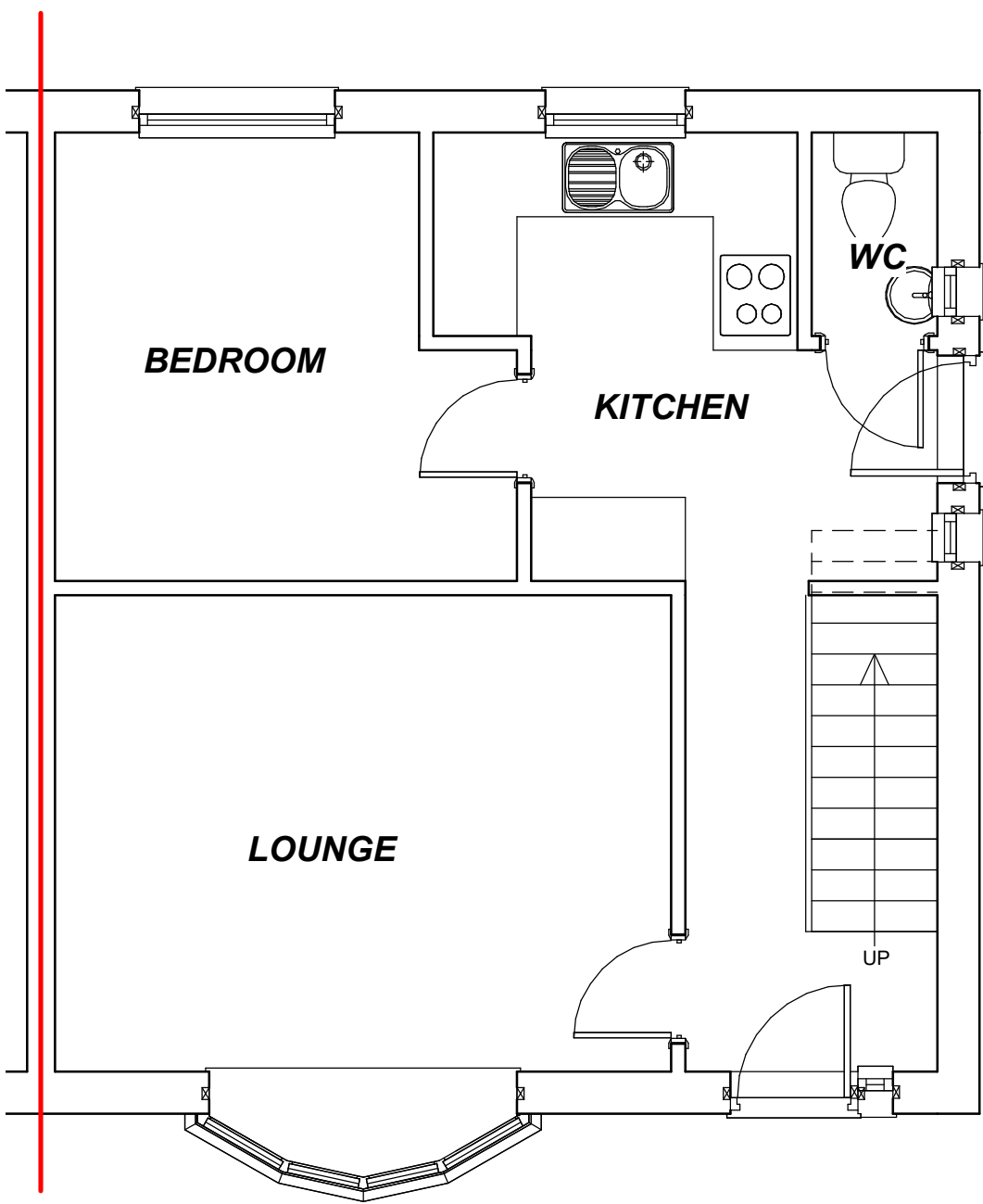
Existing Ground Floor Layout 1 : 50
