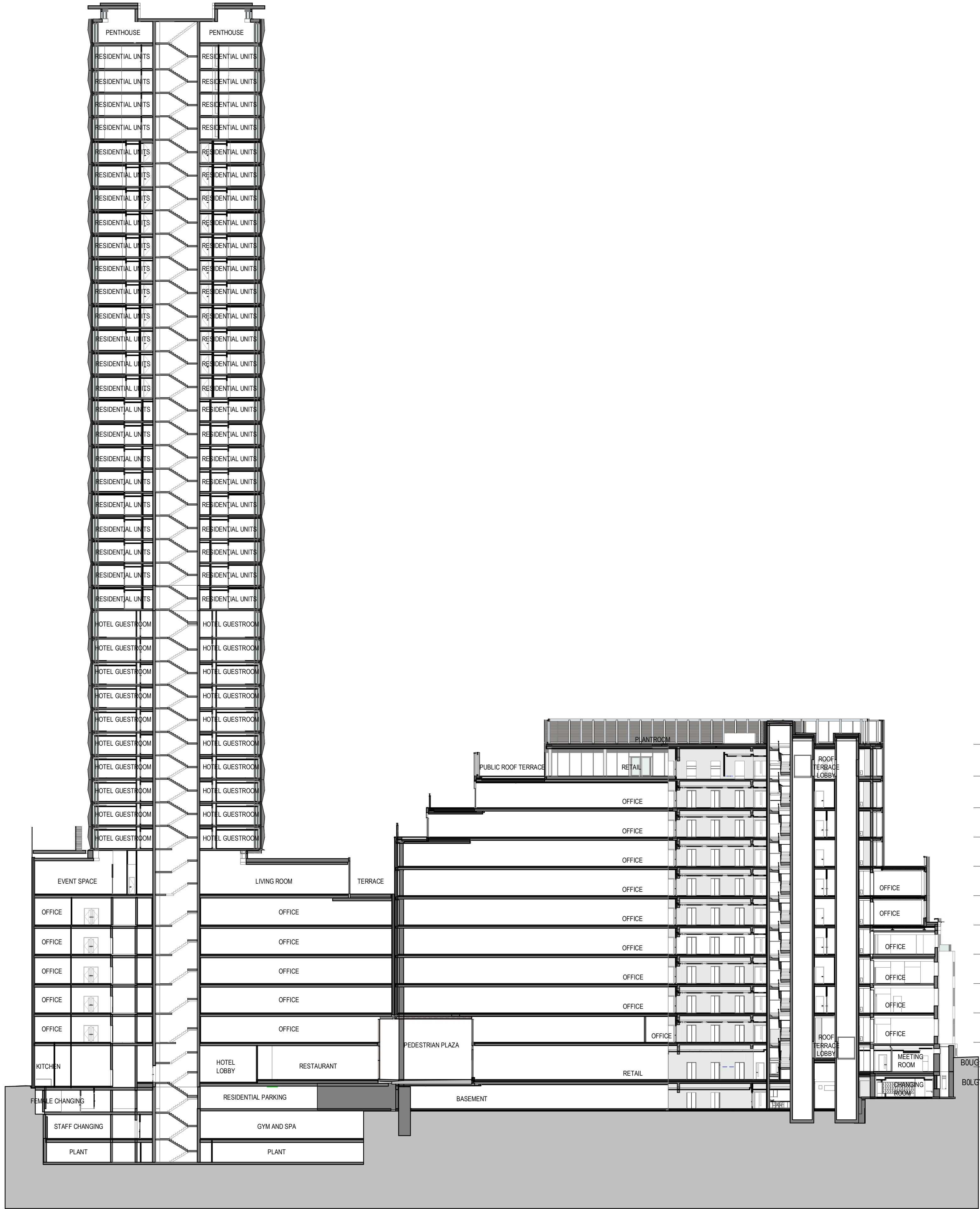
A7 CROSS SECTION WEST-EAST B 1 : 300
