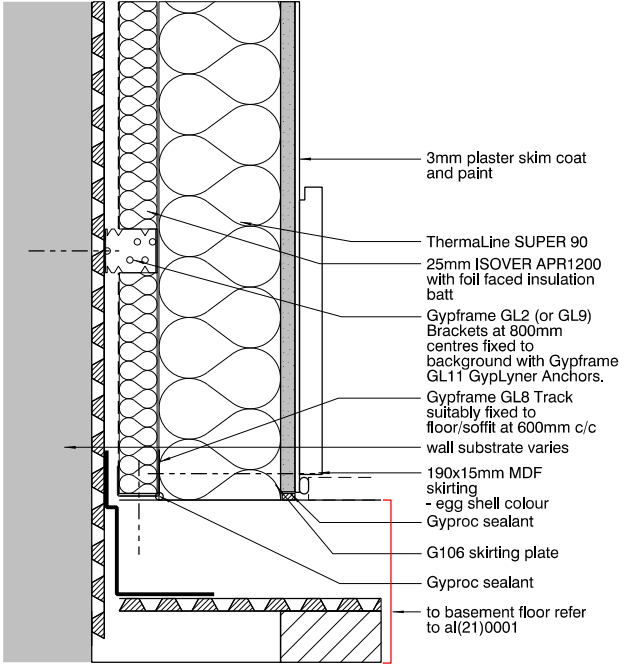
IWS-201 Bottom detail
