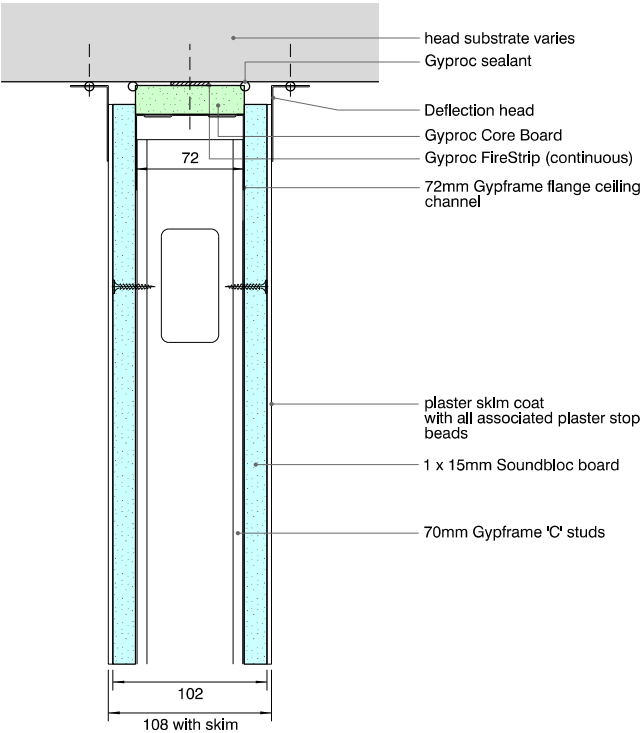
IWS-204 British Gypsum system - A206165 Fire Rating: 30 minutes Acoustic Rating Rw dB: 42
