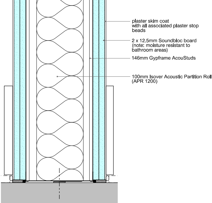
IWS-203 British Gypsum system - A206A243S Fire Rating: 60 minutes Acoustic Rating Rw (Rw + Ctr) dB: 60 (54)
