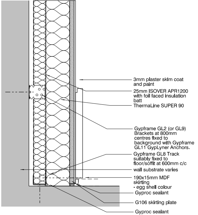
IWS-202 Bottom detail
