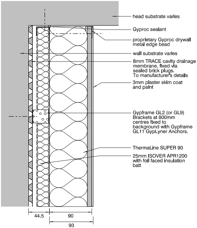
IWS-201 Head detail
