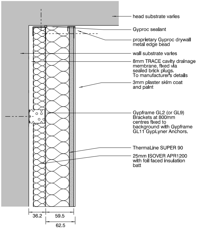
IWS-202 Head detail
