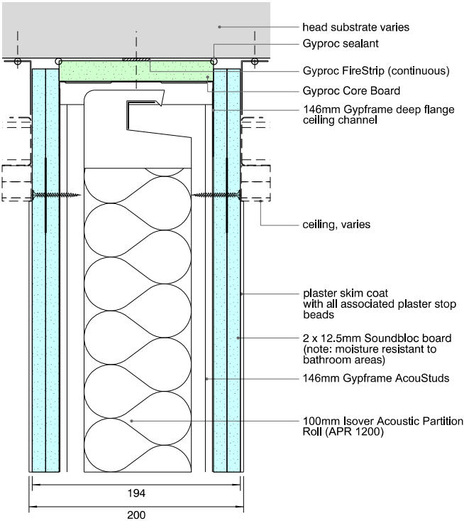
IWS-203 British Gypsum system - A206A243S Fire Rating: 60 minutes Acoustic Rating Rw (Rw + Ctr) dB: 60 (54)
