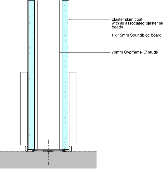
IWS-204 British Gypsum system - A206165 Fire Rating: 30 minutes Acoustic Rating Rw dB: 42
