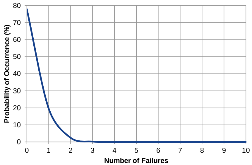
Figure 6 – Poisson distribution, probability of multiple failures
