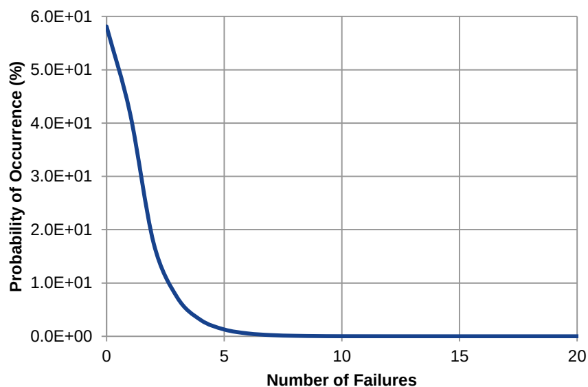
Figure 5 - Worked example, probability of multiple failures
