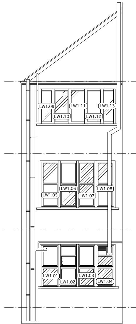
Lightwell Elevation CC Scale 1:100
