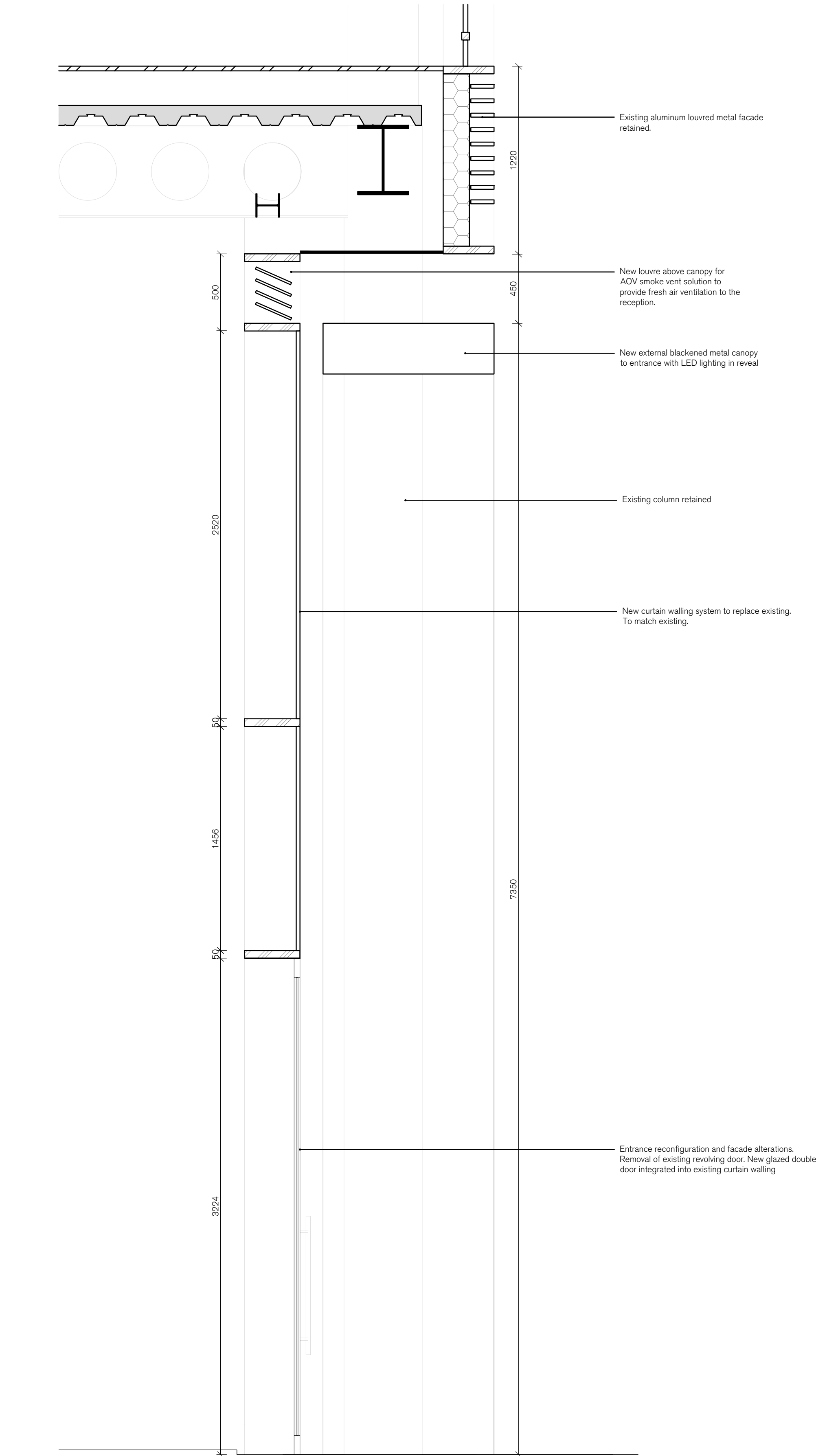
Proposed Entrance Section 1:20
