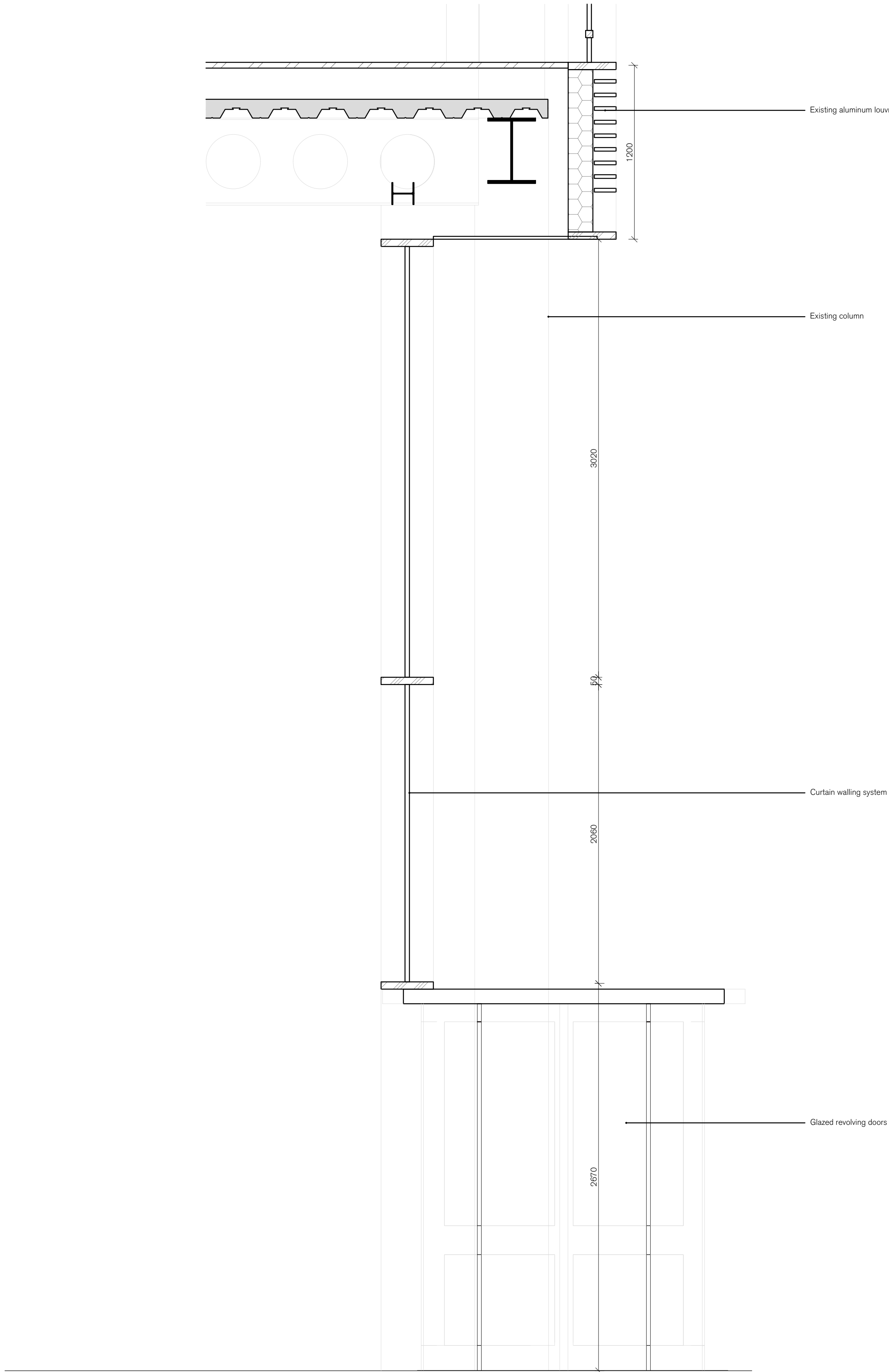
Existing Entrance Section 1:20
