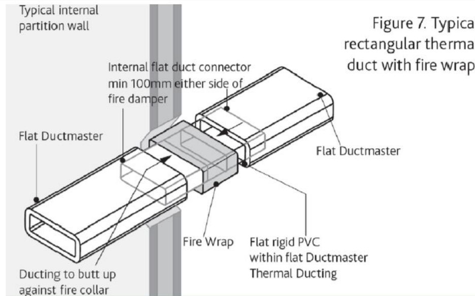
FIRE WRAP IN RECTANGULAR SLIM LINE DUCTWORK
