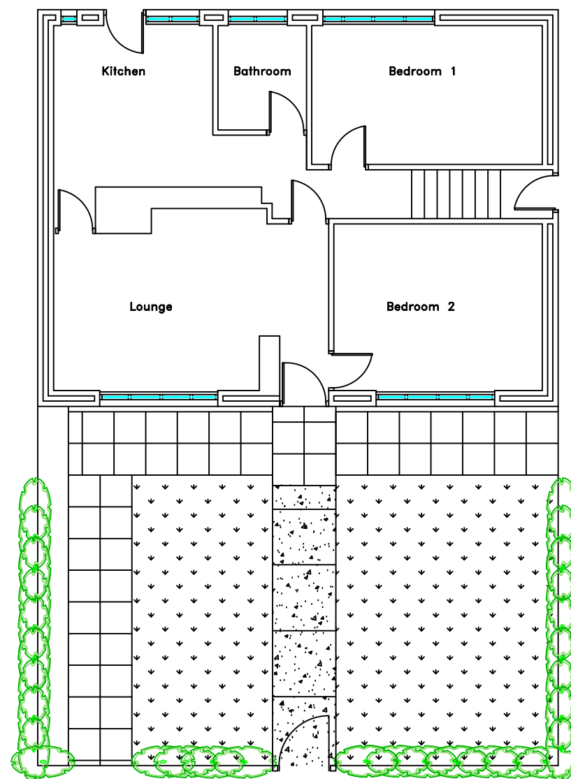
Existing Layout
