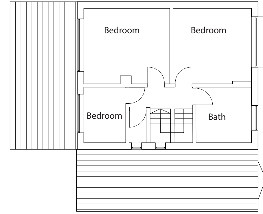
FIRST FLOOR SCALE 1:100 EXISTING - E004
