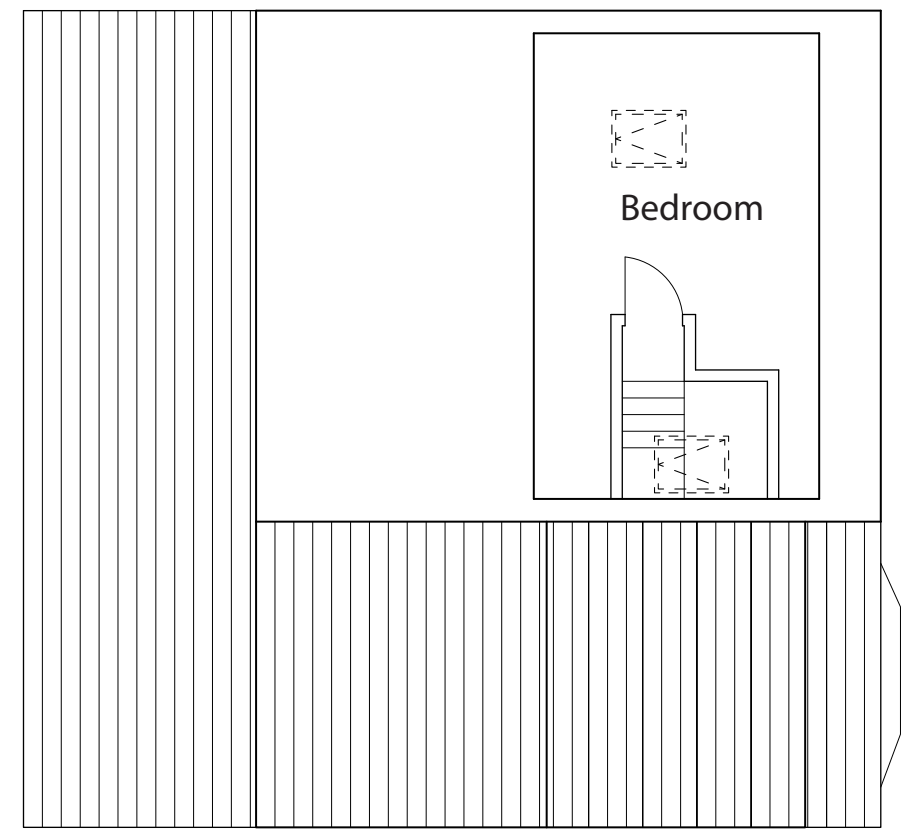
SECOND FLOOR SCALE 1:100 PROPOSED - P005
