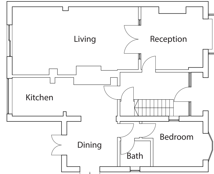
GROUND FLOOR SCALE 1:100 EXISTING - E003
