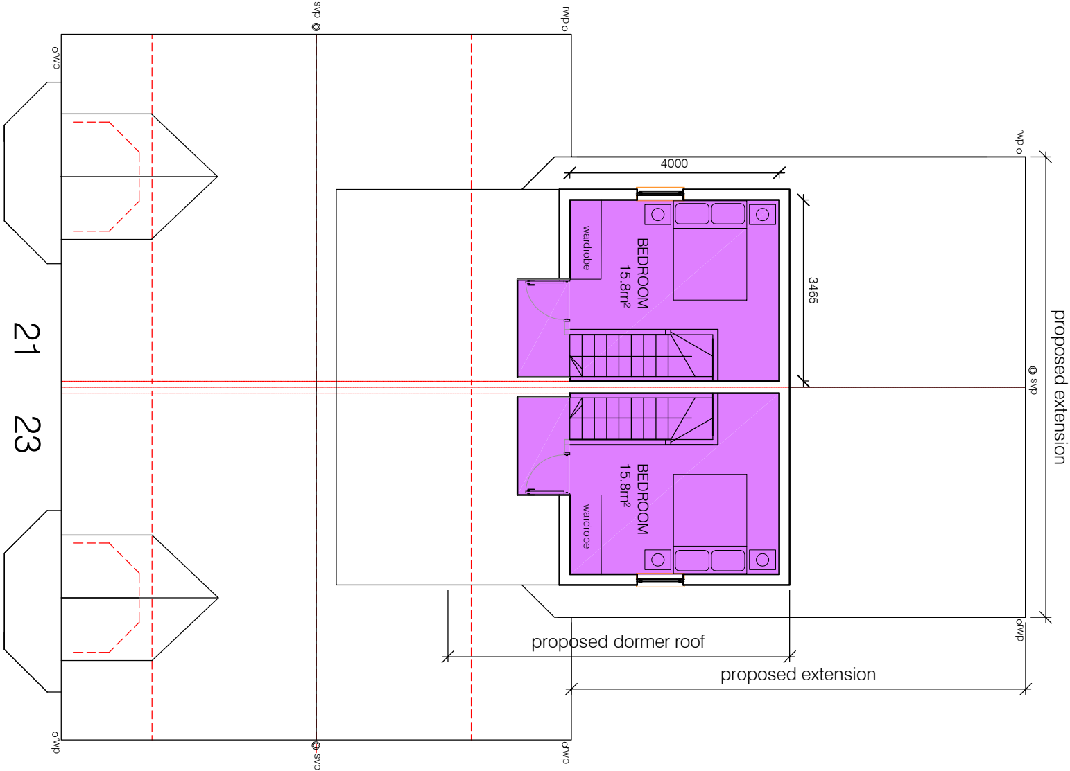
Flat 6 1B1P - 31.7m² + 15.8m² mezzanine = 47.5m² MEZZANINE/ROOF PLAN
