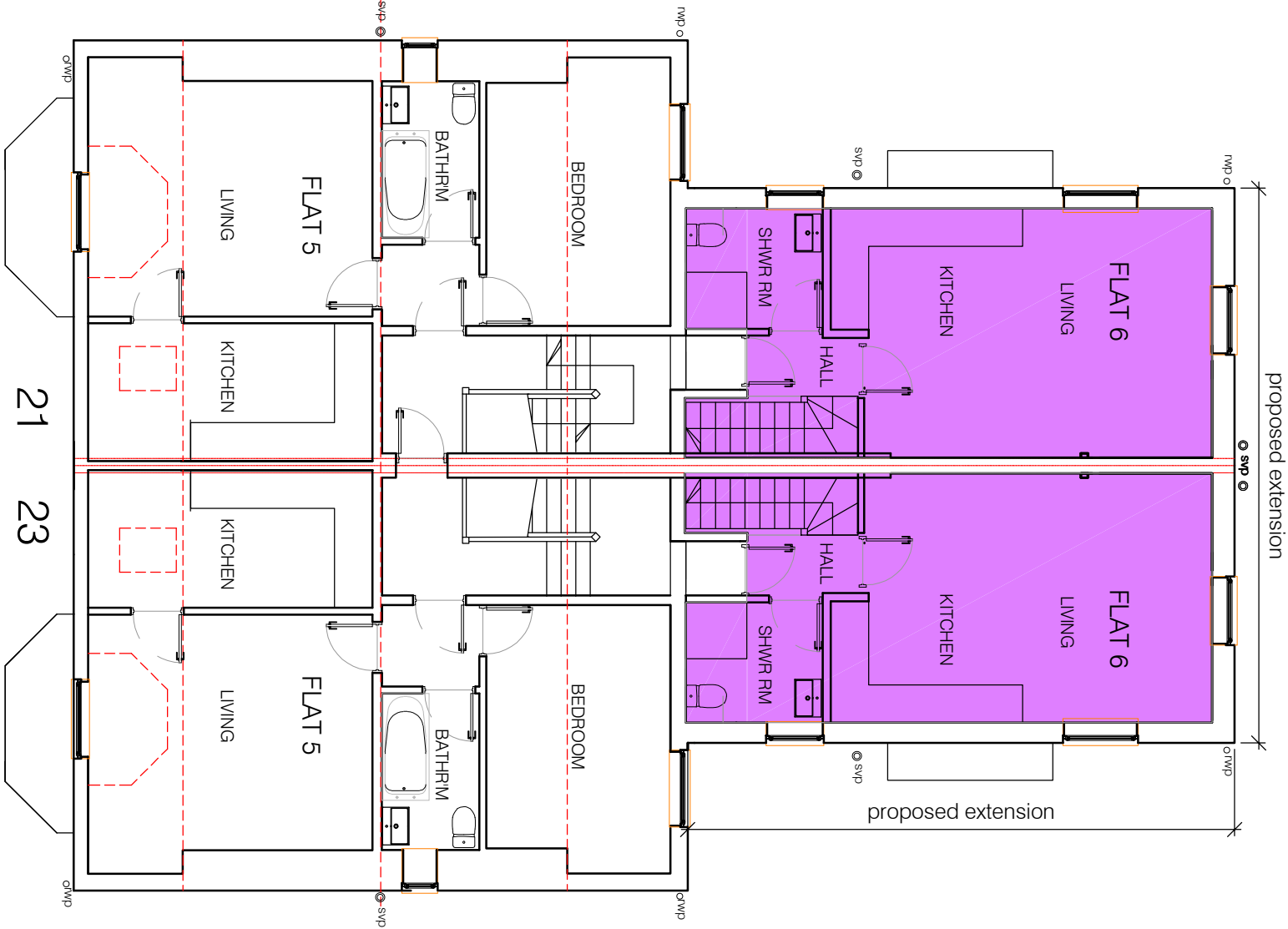
Flat 6 1B1P - 31.7m² + 15.8m² mezzanine = 47.5m² SECOND FLOOR PLAN
