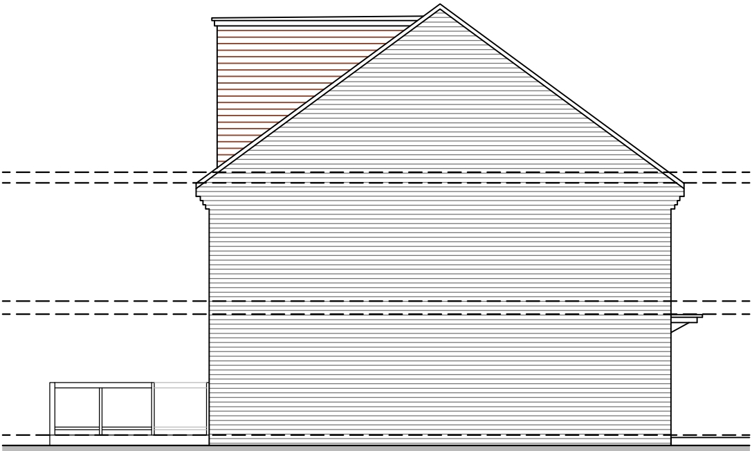
SIDE ELEVATION 1:100
