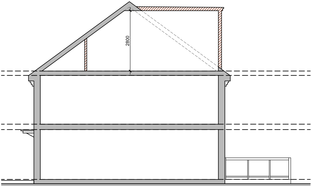
SECTION 1:100
