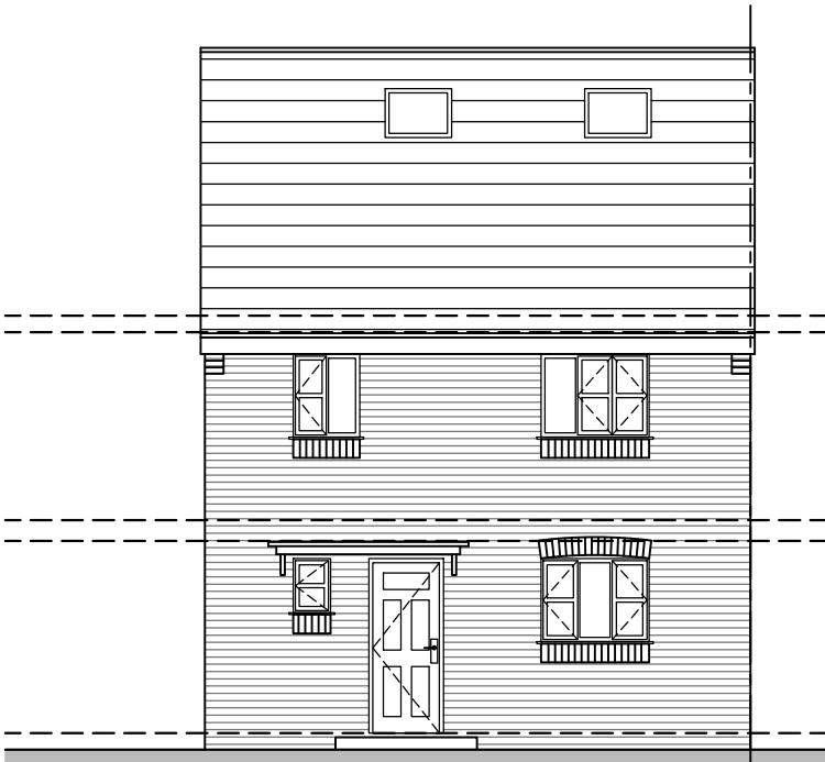
FRONT ELEVATION 1:100
