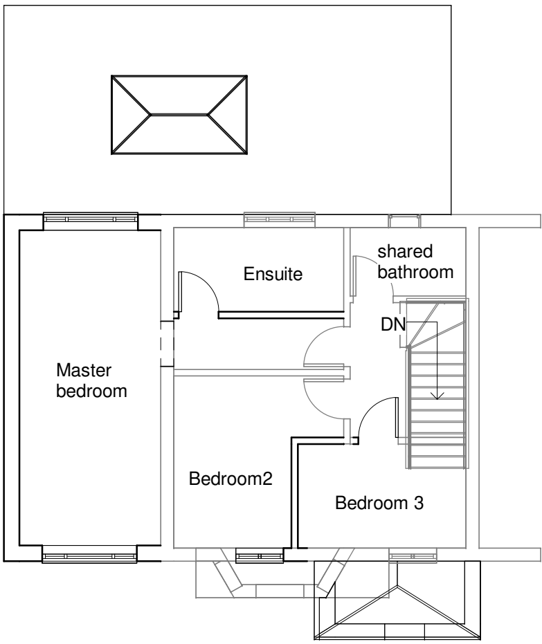
4 FF- Proposed 1 : 100
