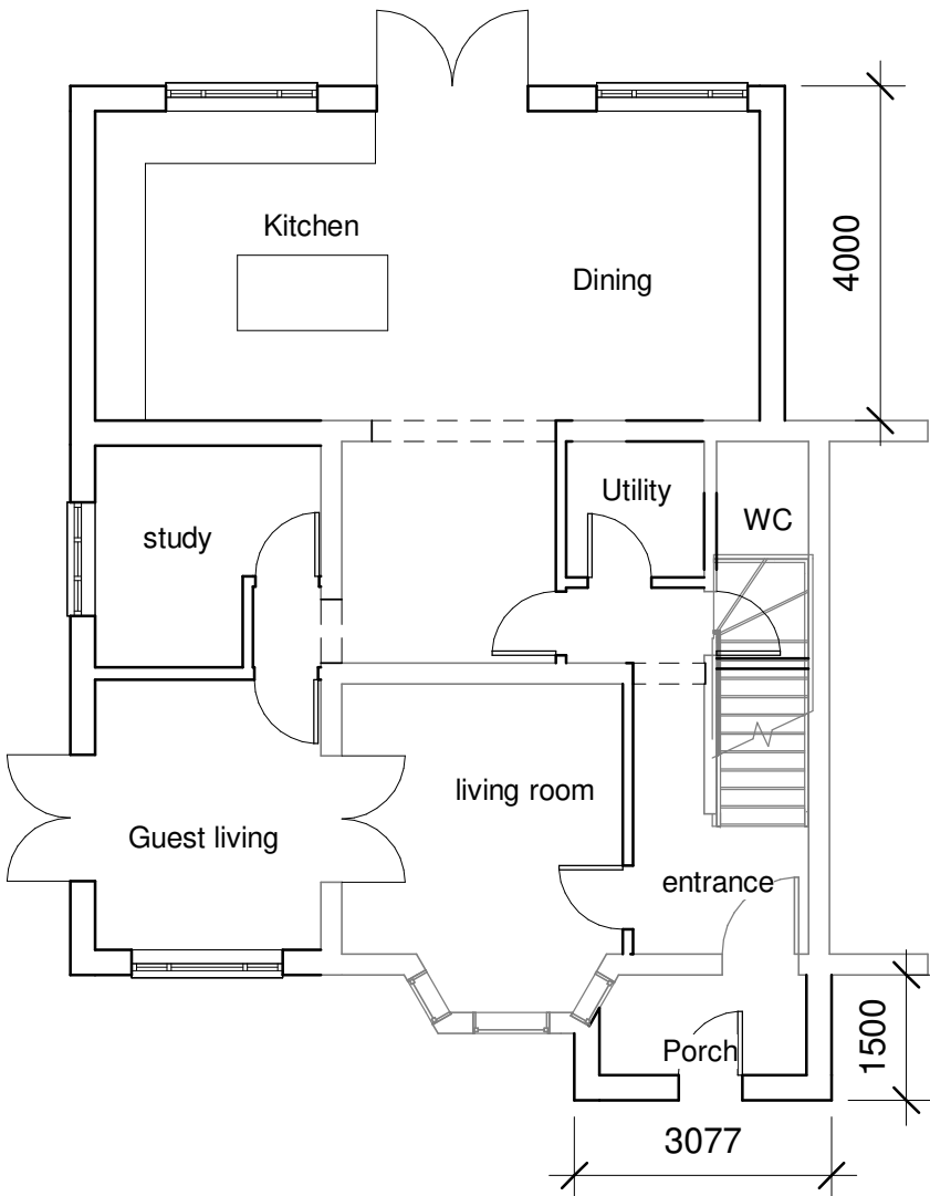
2 GF- Proposed 1 : 100
