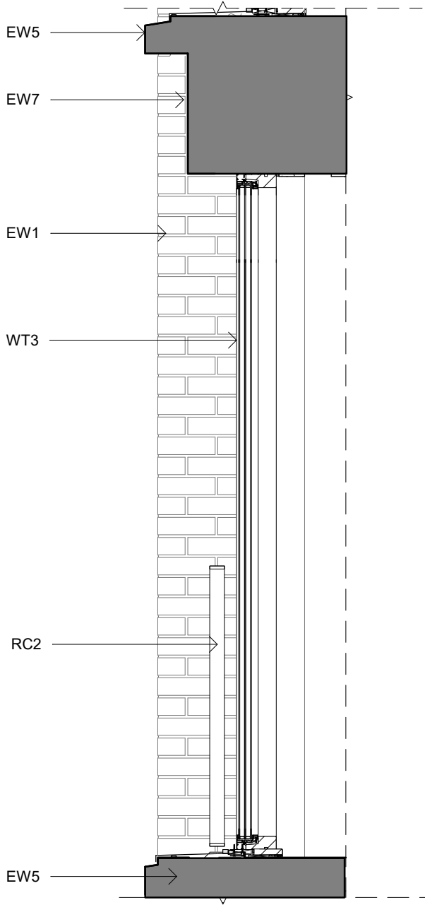
1-20 Detail Sections - Sample Panel 1 : 20
