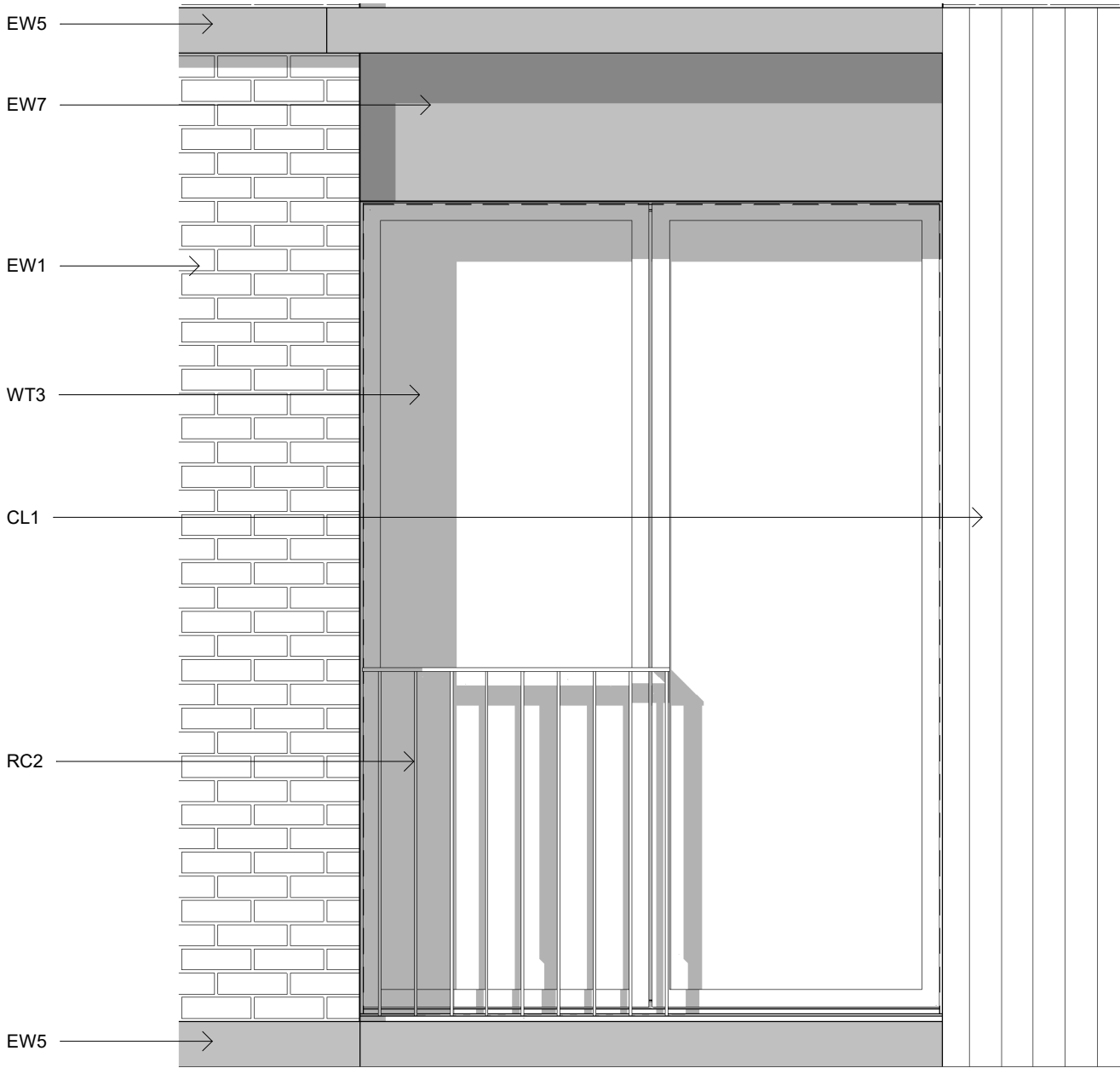
Typical Residential Window_Sample Panel 1 : 20
