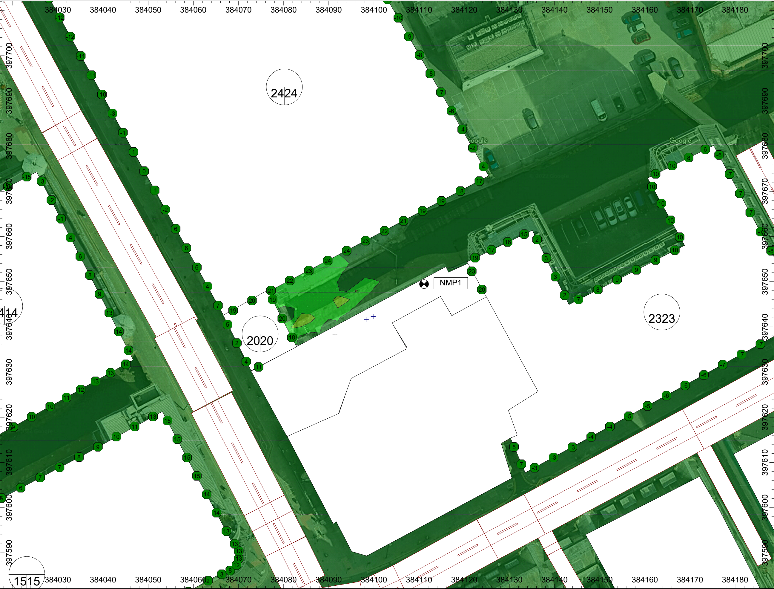
Figure 2 - Fixed Plant Sound Grid Noise Map - Calculation at 15m above ground level
