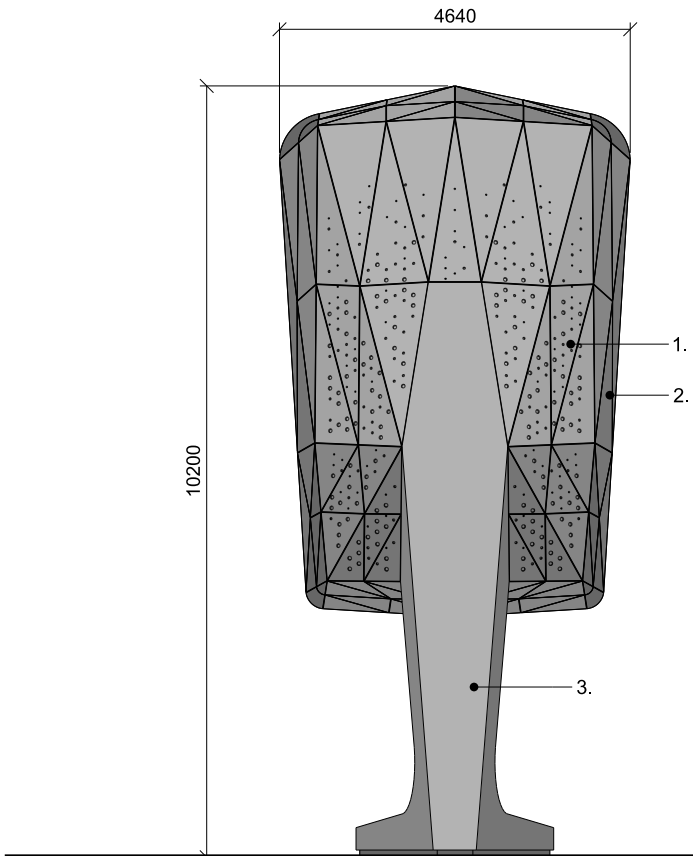
REAR ELEVATION
