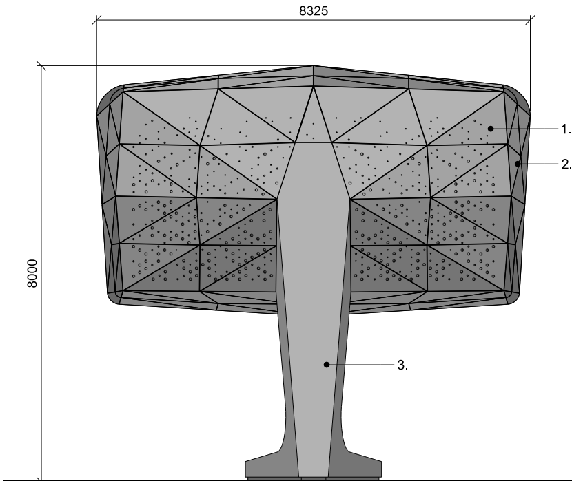
REAR ELEVATION
