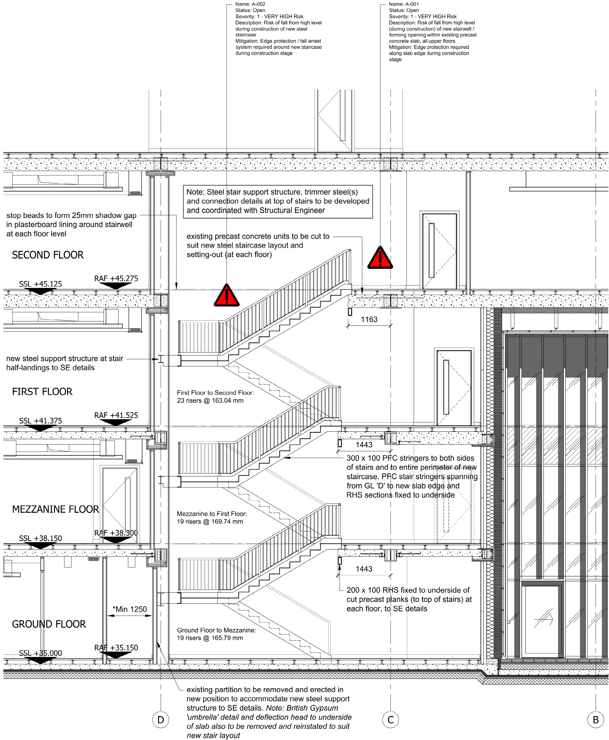
PROPOSED CROSS SECTION THROUGH NEW STAIRCASE SCALE 1:50
