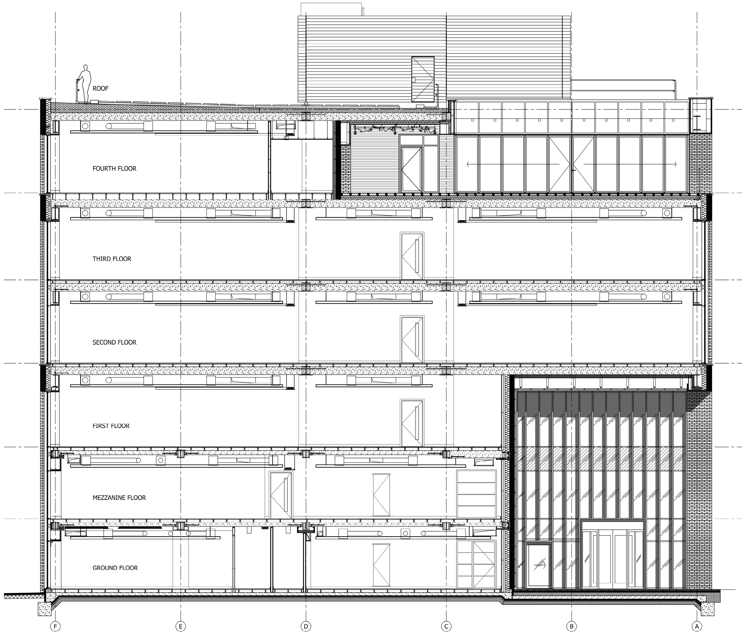
EXISTING CROSS SECTION SCALE 1:100
