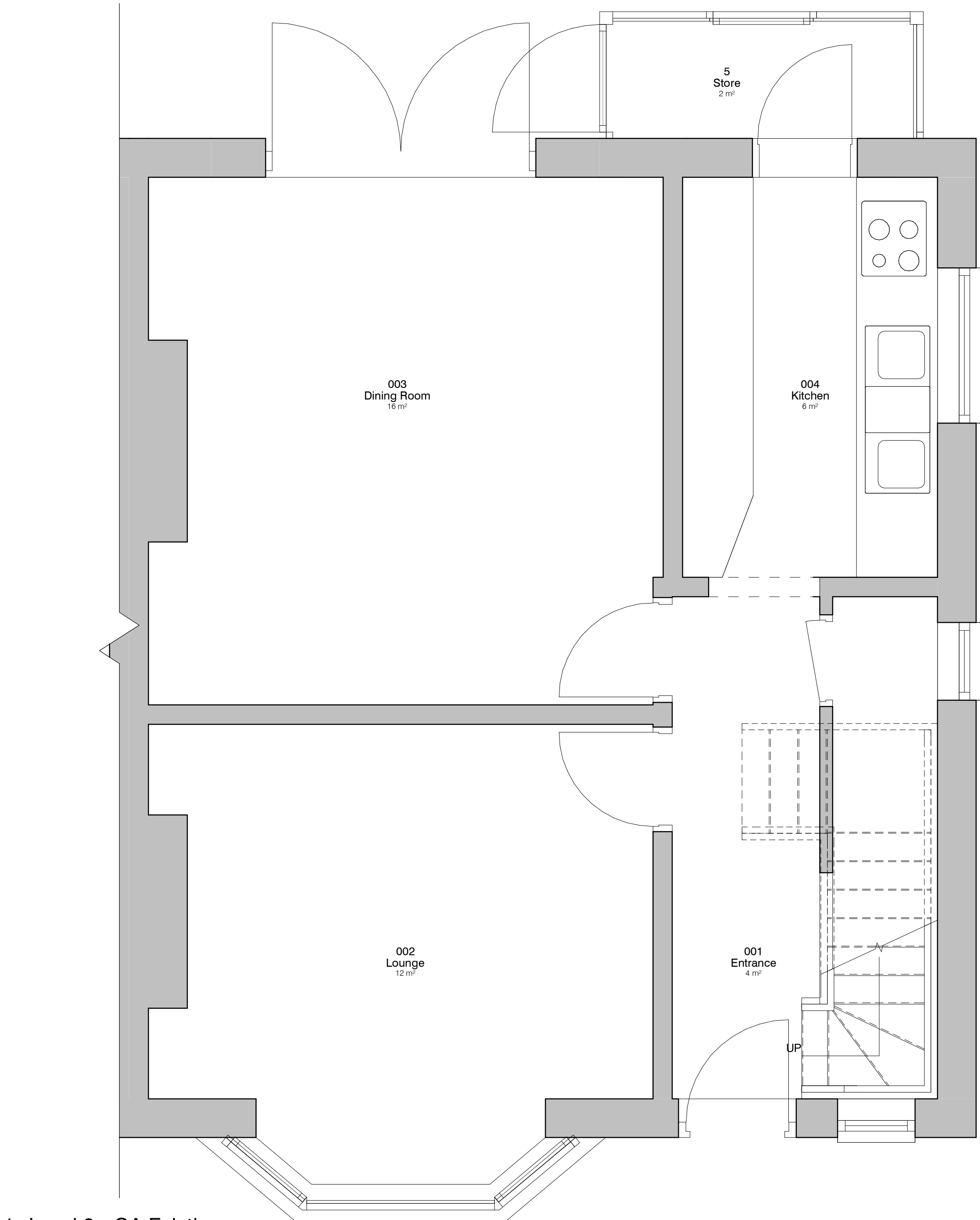
1. Level 0 - GA Existing 1 : 25
