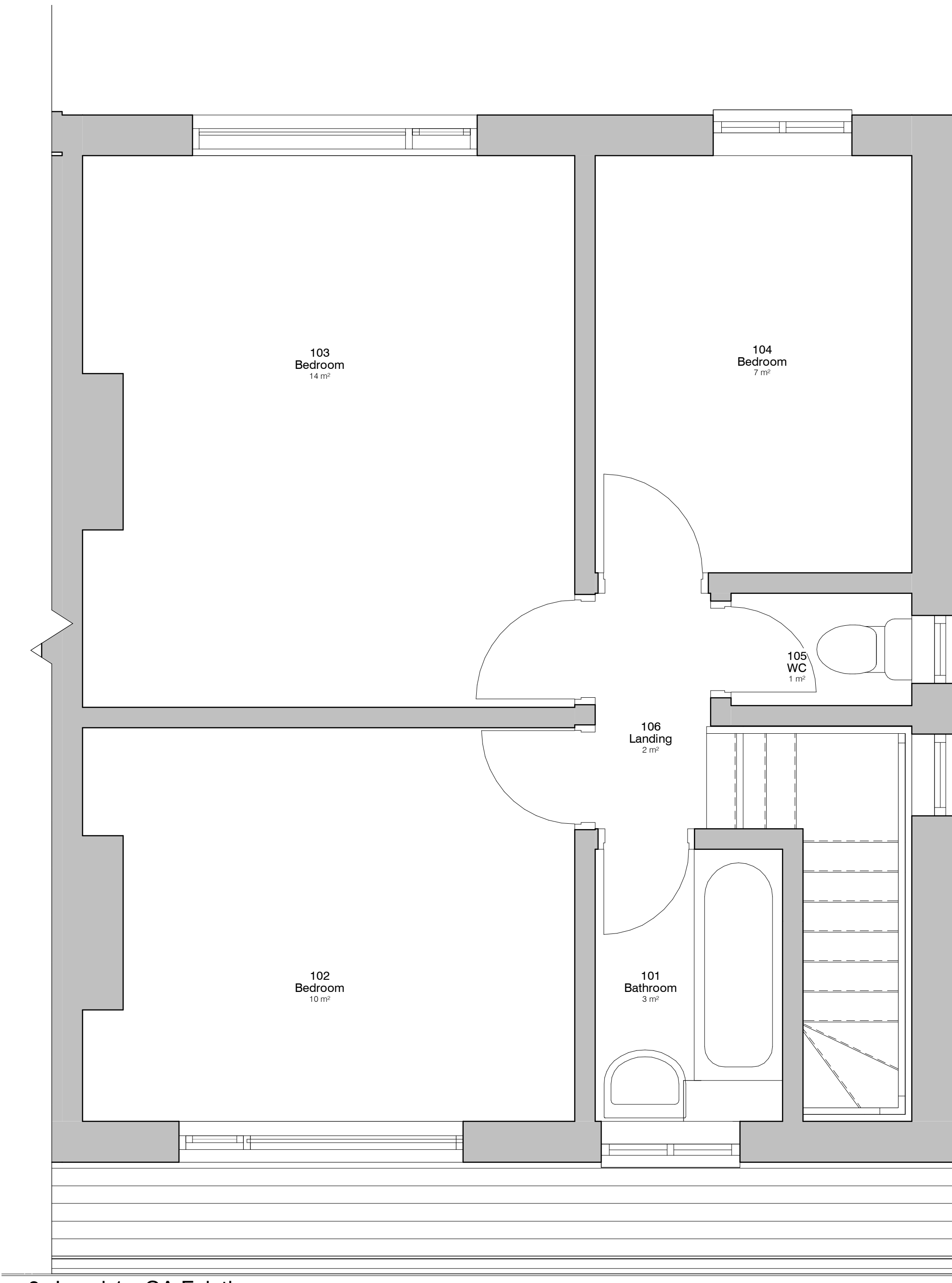
2. Level 1 - GA Existing 1 : 25
