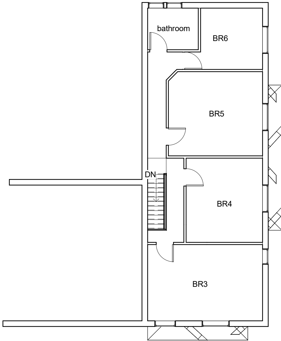
3 First Floor- Existing 1 : 100
