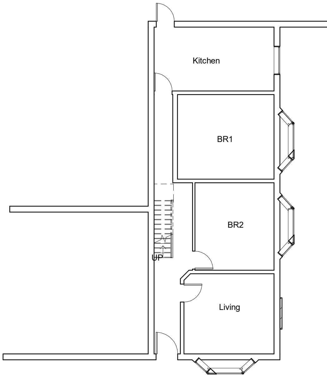
1 Ground Floor- Existing 1 : 100
