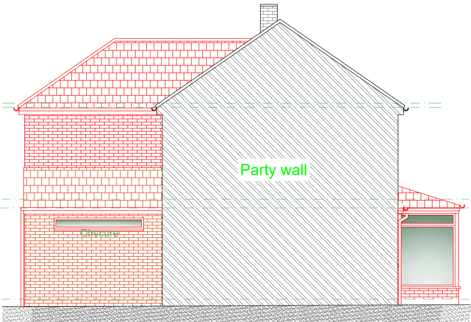
Proposed L/H Side Party Wall Elevation Scale 1:100
