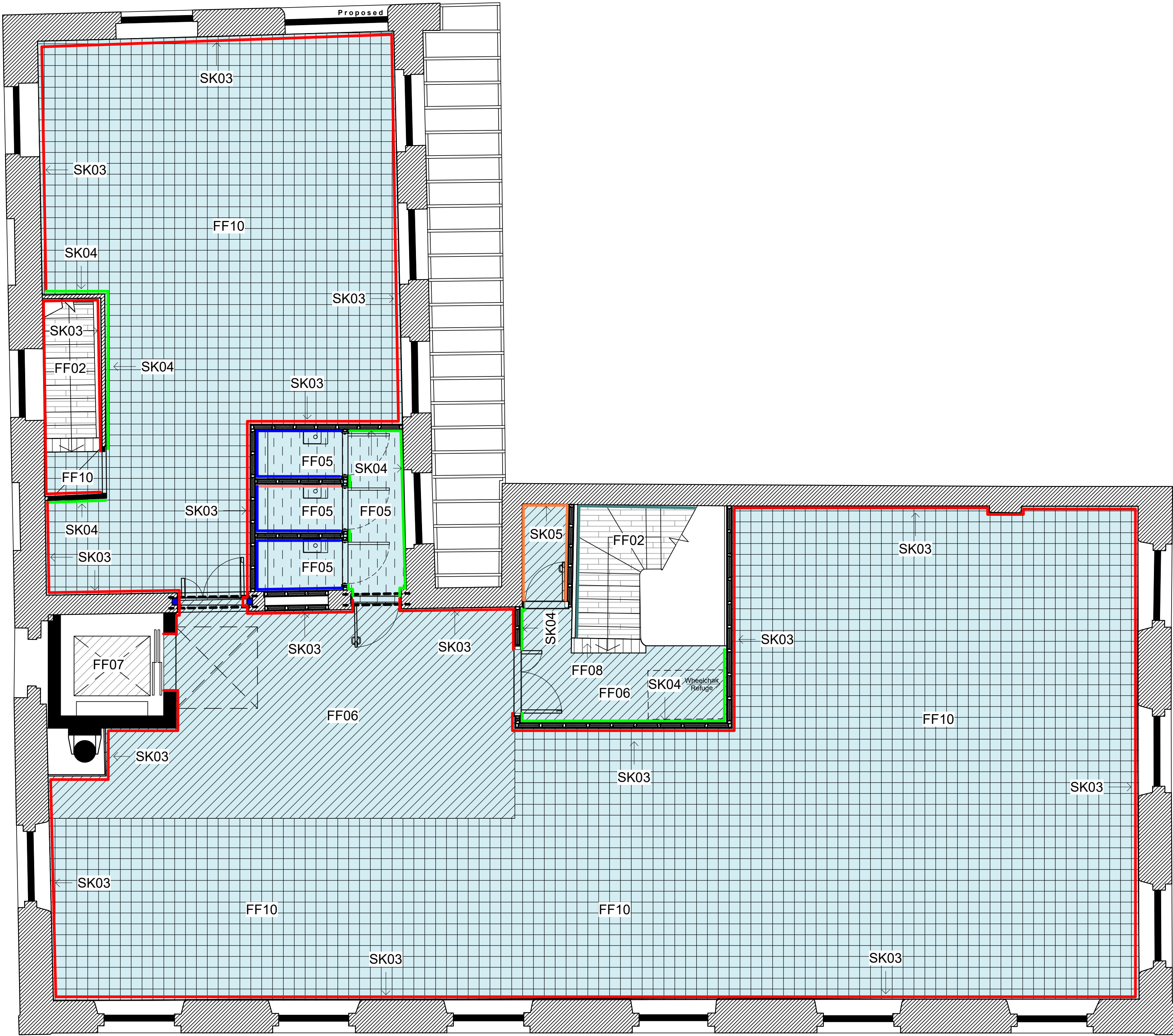
4FL Proposed Floor Finishes 1 : 50
