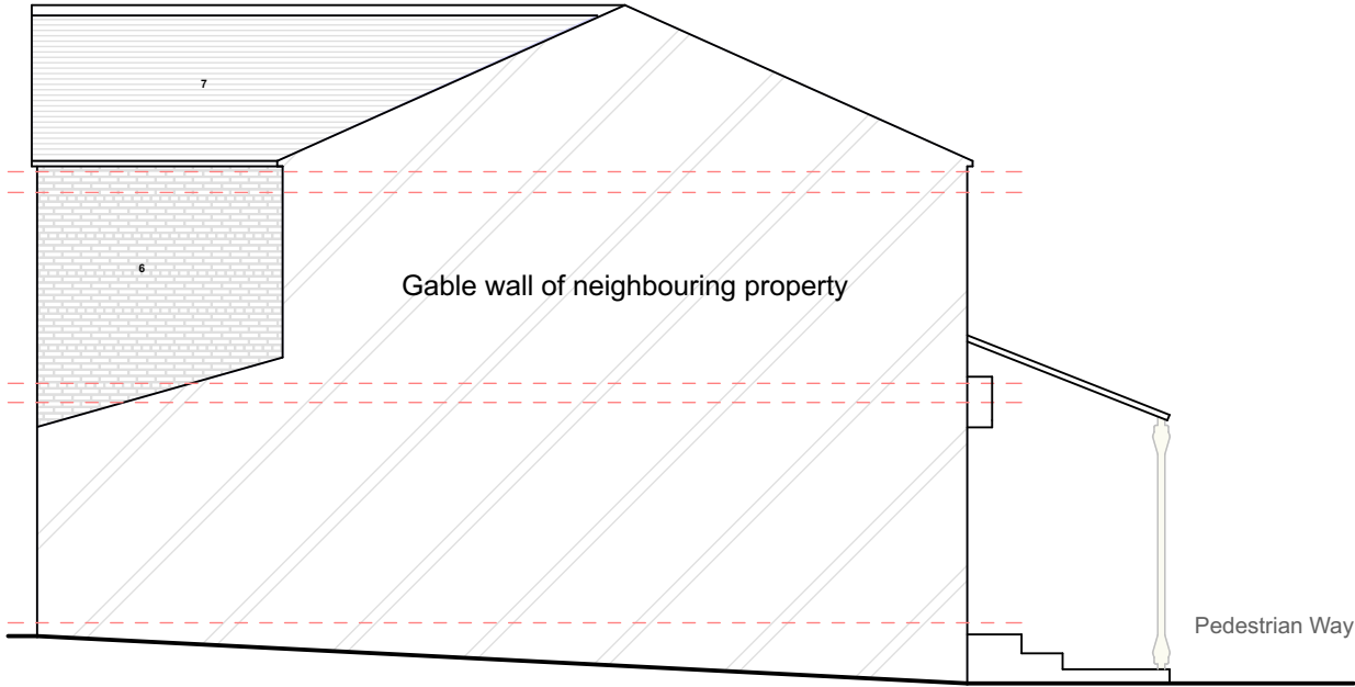
PROPOSED GA SIDE ELEVATION 1 @1:100
