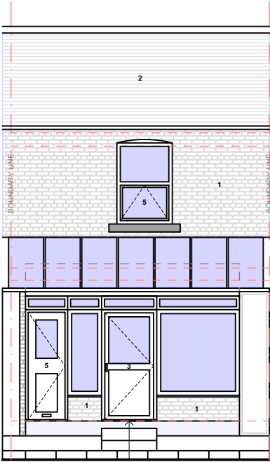
PROPOSED GA FRONT ELEVATION @1:100
