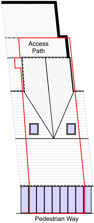
PROPOSED GA SITE PLAN @1:200
