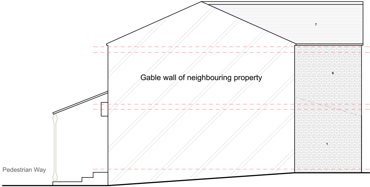
PROPOSED GA SIDE ELEVATION 2 @1:100
