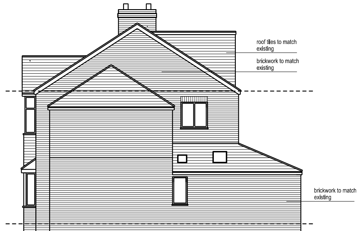
North Elevation
