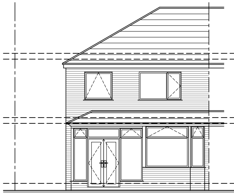
FRONT ELEVATION
