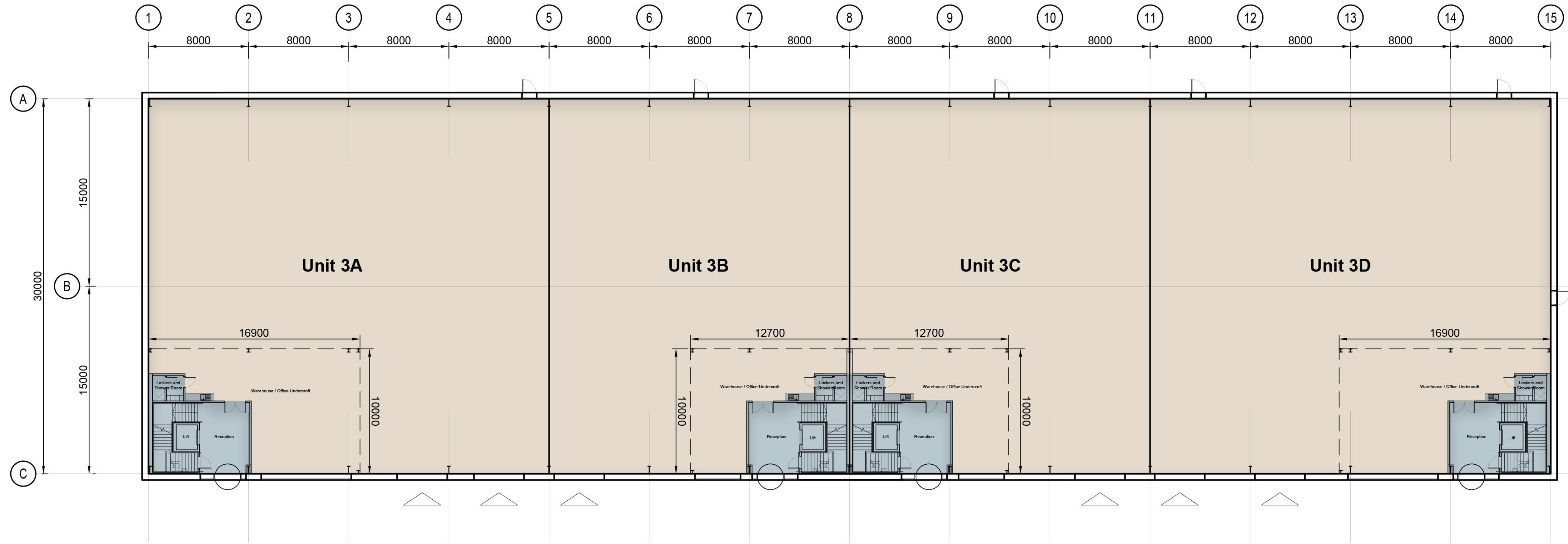
Ground Floor Building Plan 1:200
