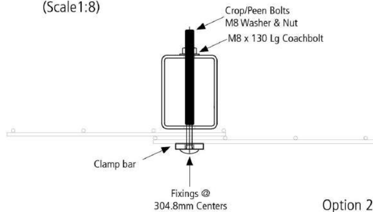
Mesh Clamp Detail (Scale 1:8)
