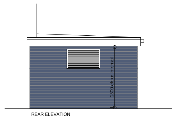
Elevations 1:100
