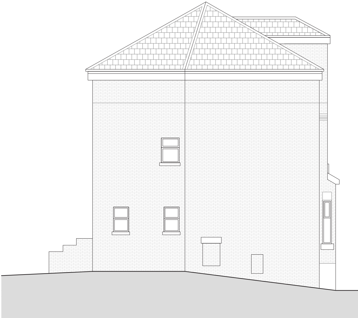
EXISTING SIDE ELEVATION 1:100 @ A3
