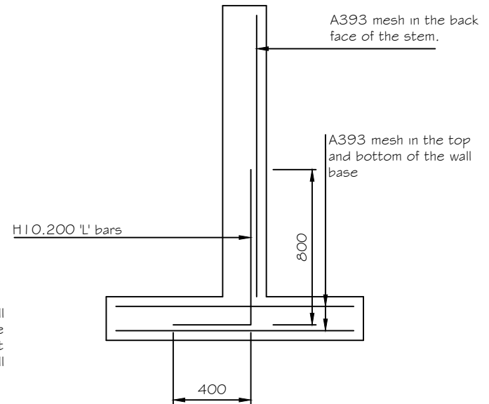
REBAR DETAILS AND WALL TIES 1:20
