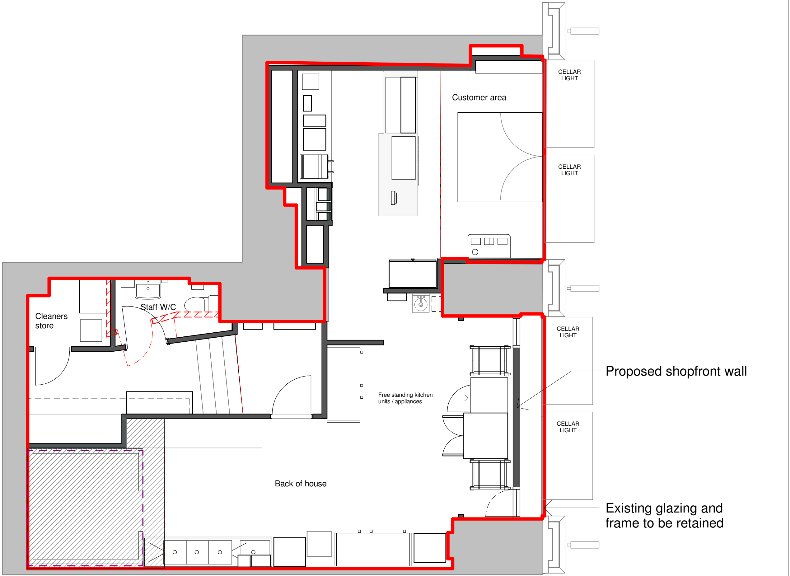
Ground floor plan - proposed layout with shopfront window display 1 : 50
