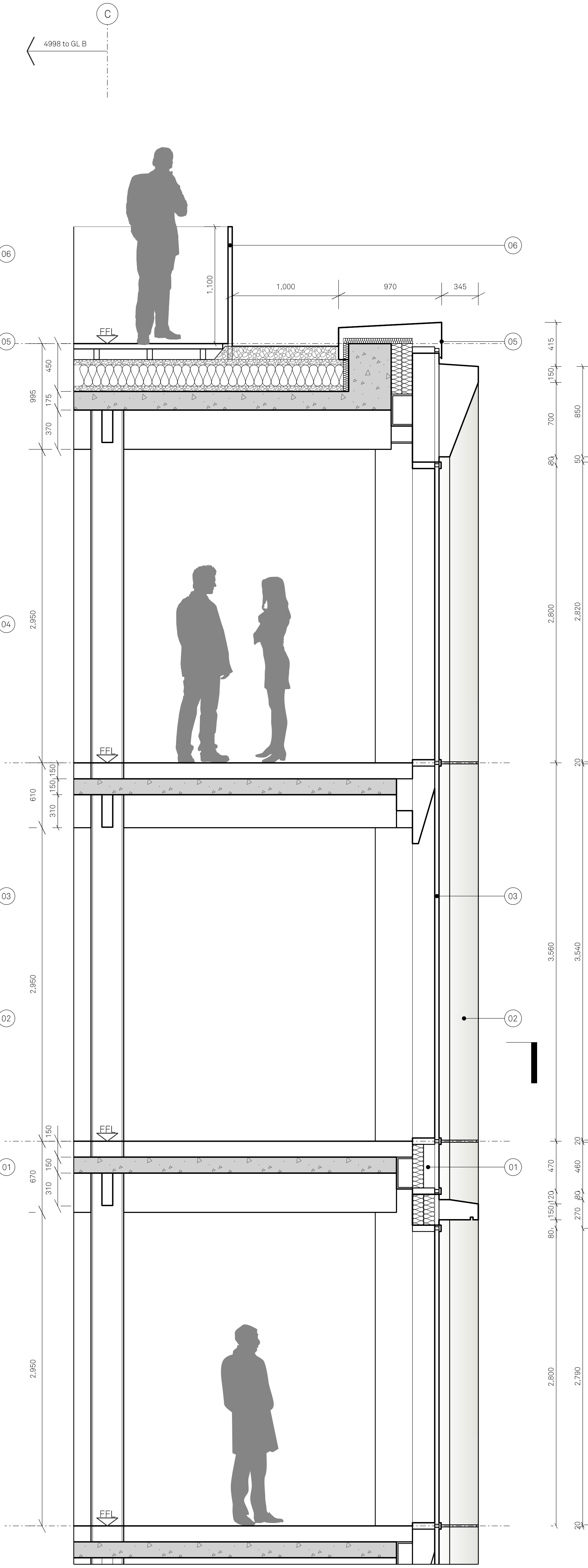
SECTION A Office Levels and Roof Terrace
