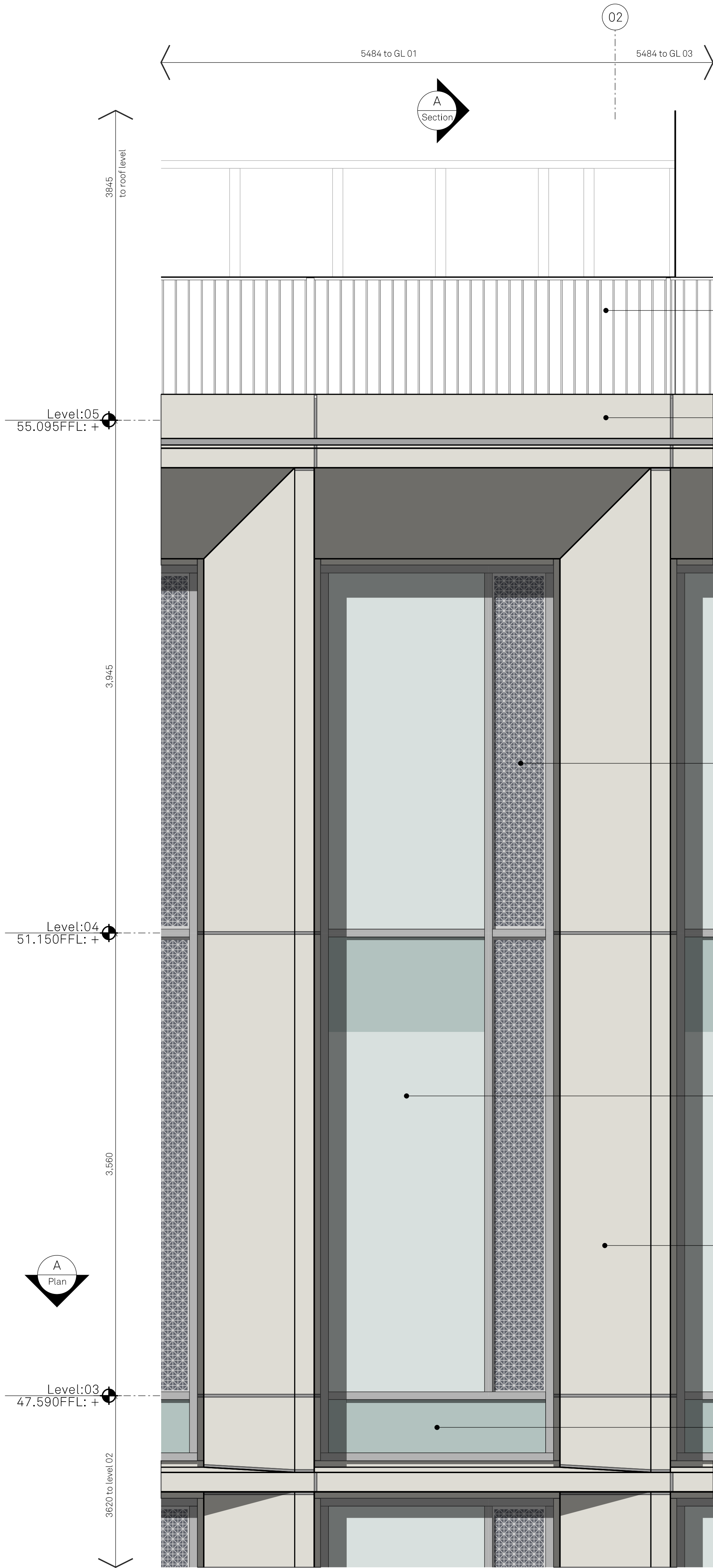
PARTIAL ELEVATION Upper Levels & Roof Terrace
