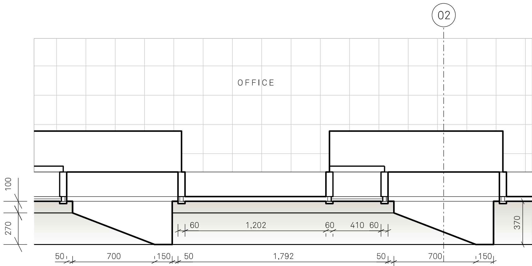
PLAN A Typical Office Level
