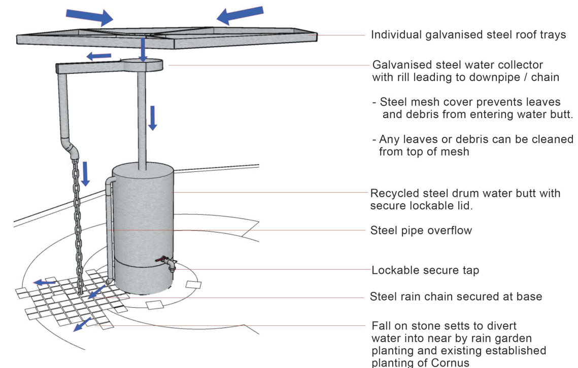
WATER CIRCULATION
